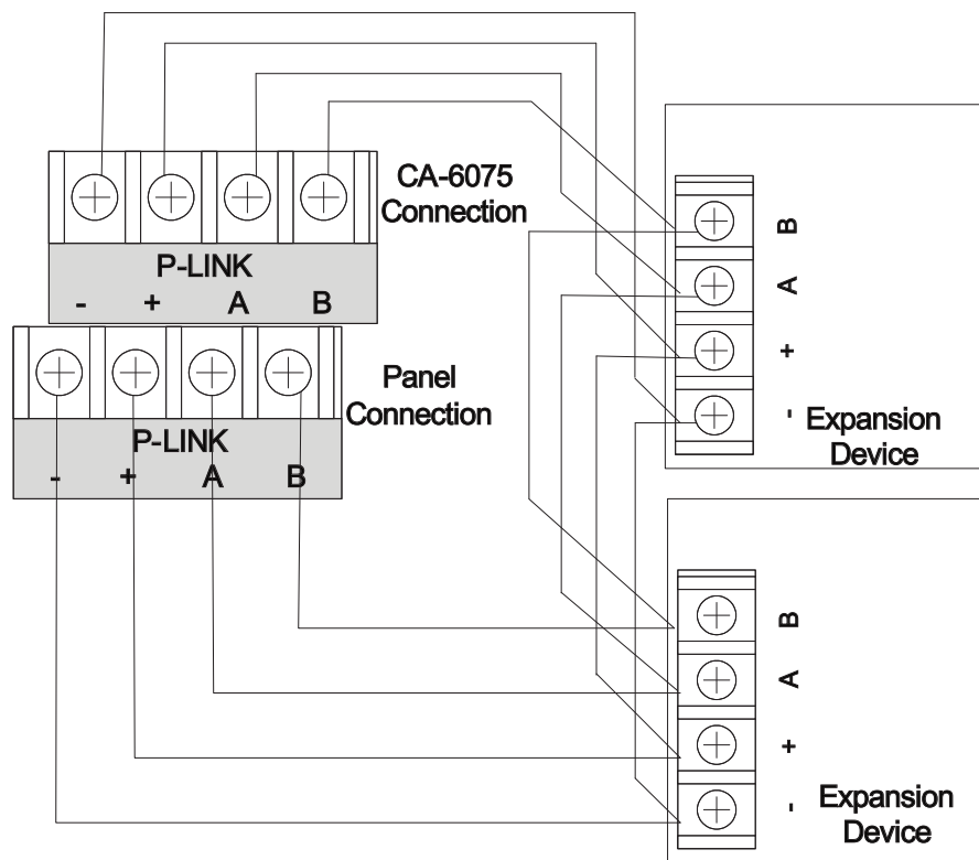
Figure 13. Example of P-Link Class B Wiring
