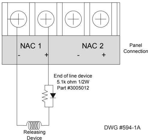
Figure 15. NAC Releasing Circuit Wiring with EOLD Assembly
