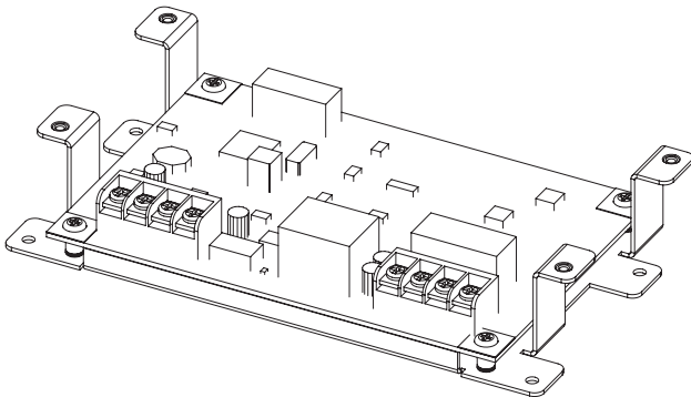
Figure 21. PAD100-SLCE / SLCE-127 Board & Shown Installed in accessory cabinet
