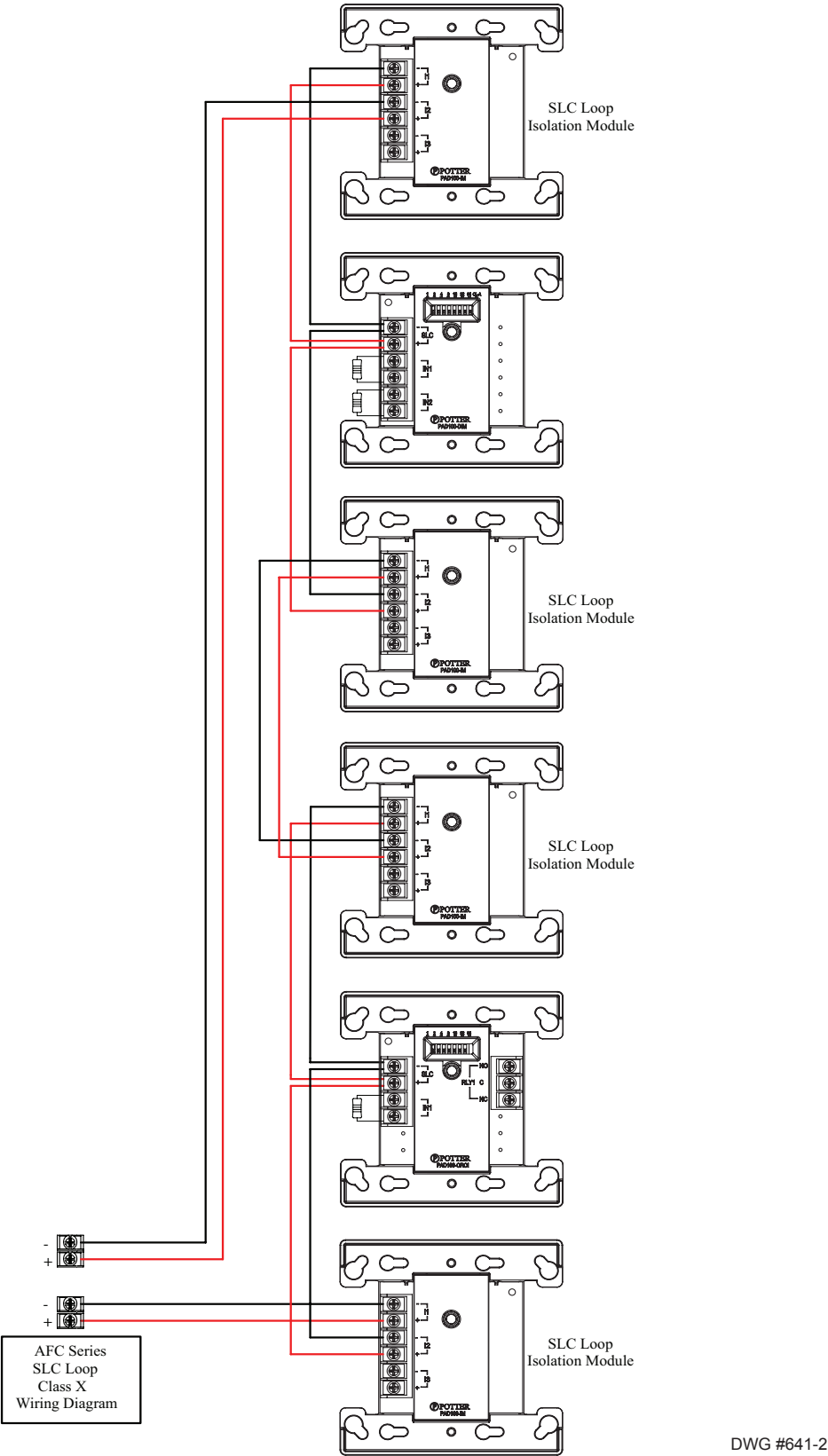
Figure 7. PAD Protocol Class X Showing PAD100-IMs Installed
