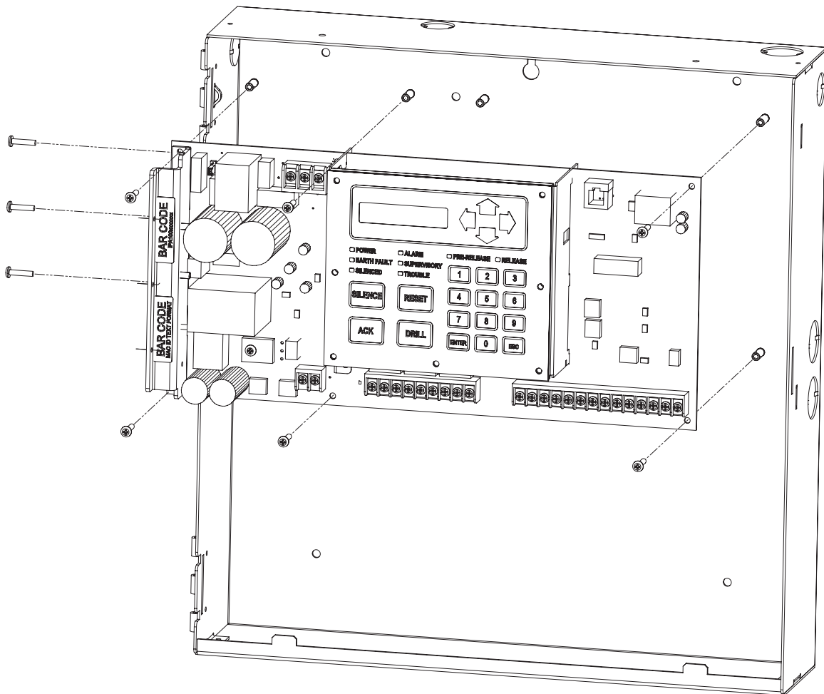
Figure 34. AFC-50 Cabinet Showing Circuit Board Assembly
