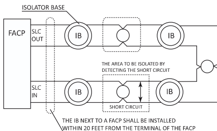
FIGURE 3: Wiring (Class X) Using PAD100-IB
