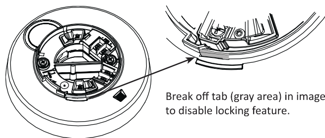
FIGURE 12: Disable Locking Feature
