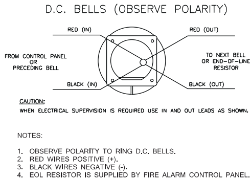
FIGURE 2. PDC BELL MOUNTING
