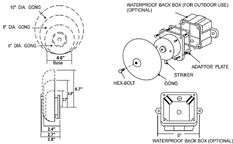
FIGURE 2. PDC BELL MOUNTING
