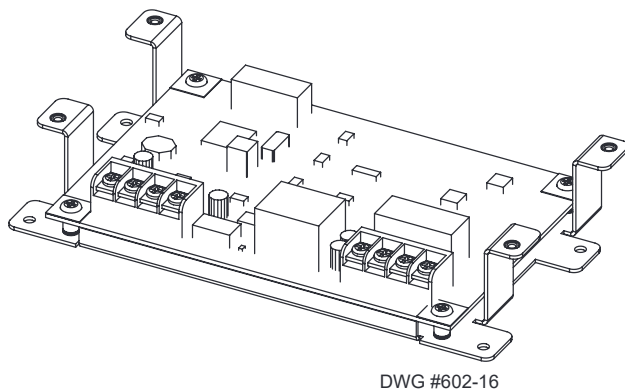
Figure 21. PAD100-SLCE / SLCE-127 Board &amp; Showing Mounting Bracket
