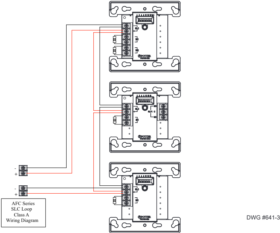
Figure 8. PAD Protocol Example of SLC as Class A
