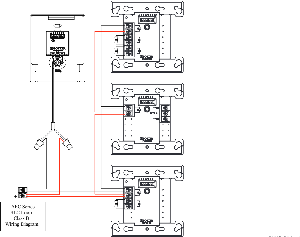
Figure 9. PAD Protocol Example of SLC as Class B
