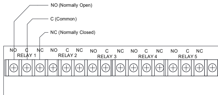
Figure 41. RLY-5 Wiring to Control Panel /Auxiliary Power Supply Examples & RLY-5 Showing Normally Open/Normally Closed Contacts
