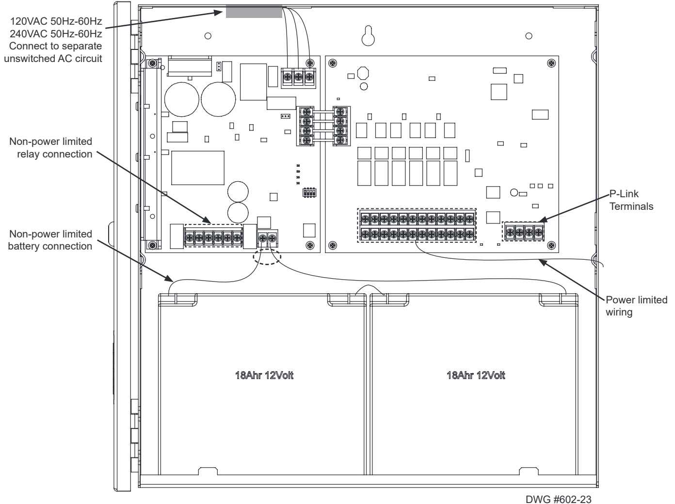
Figure 66. PSN-1000E Wiring
