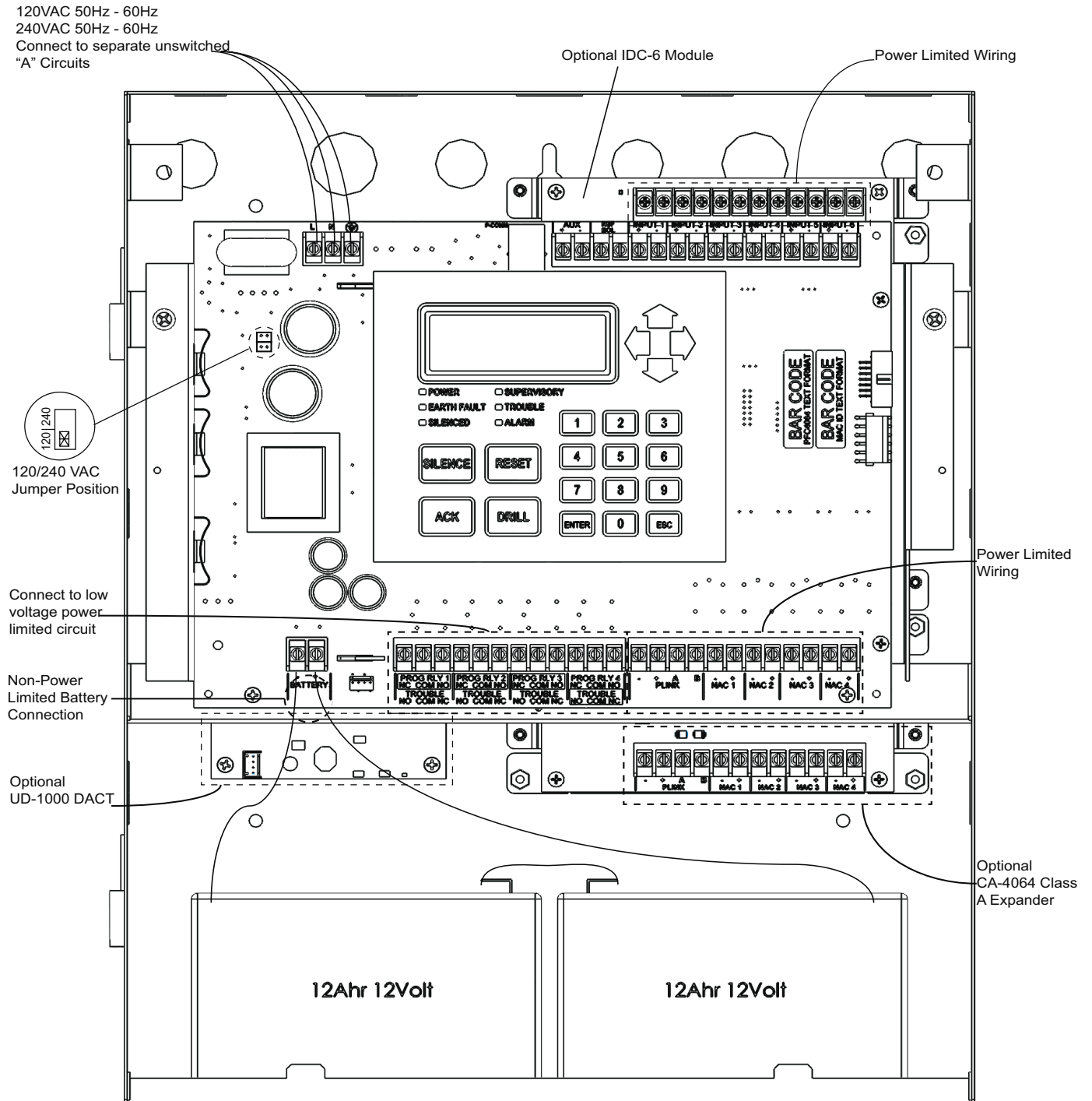
Figure 3. PFC-4064 Cabinet Wiring --
