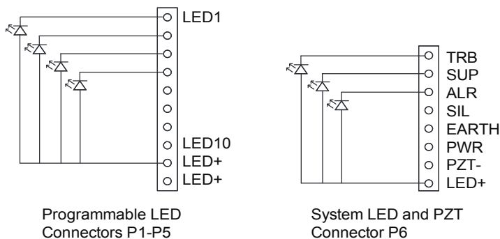
Figure 36. DRV-50 "P1-P5" and "P6" Connectors
