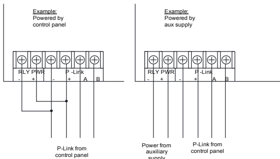
Figure 41. RLY-5 Wiring to Control Panel /Auxiliary Power Supply Examples & RLY-5 Showing Normally Open/Normally Closed Contacts
