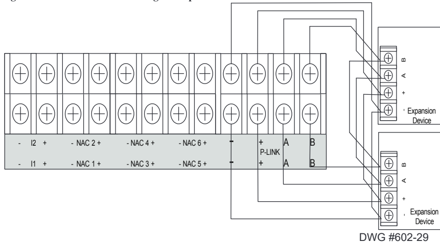
Figure 72. P-Link Class A Wiring Example
