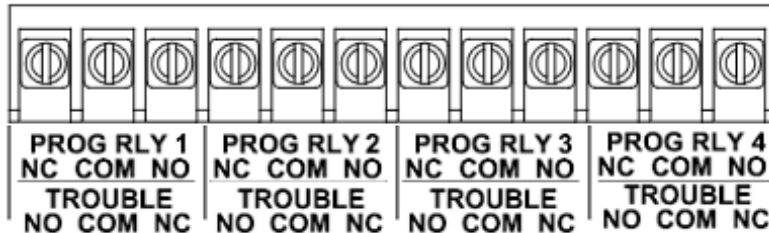
Figure 12. Relay Output Wiring
