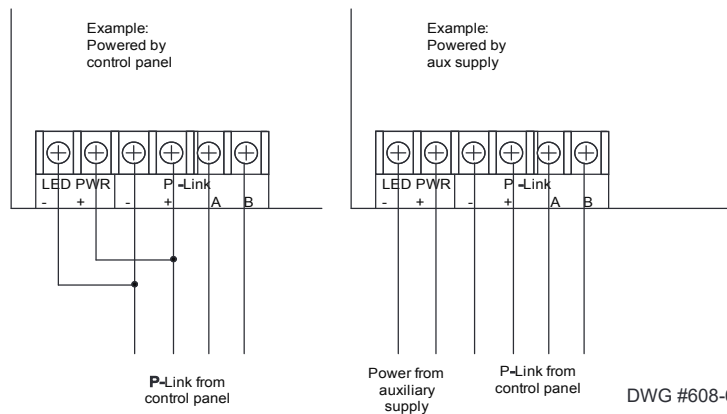
Figure 38. Examples of Wiring DRV-50 from Control Panel or Auxiliary Power Supply
