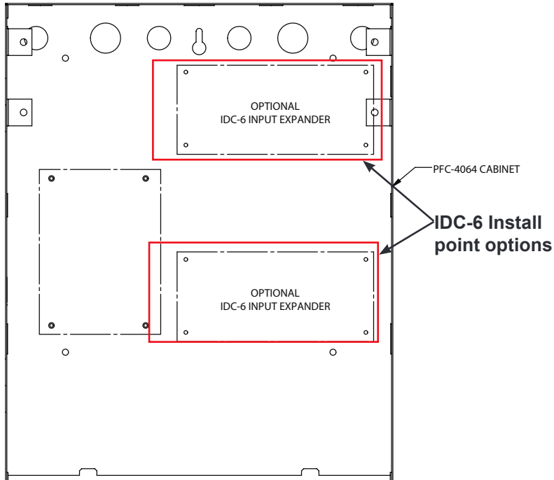
Figure 21. IDC-6 Module locations
