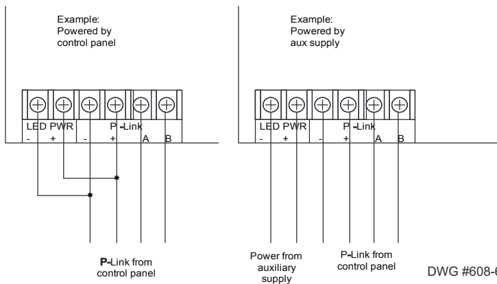
Figure 33. Examples of Wiring LED-16 Module to Control Panel or Auxiliary Power Supply
