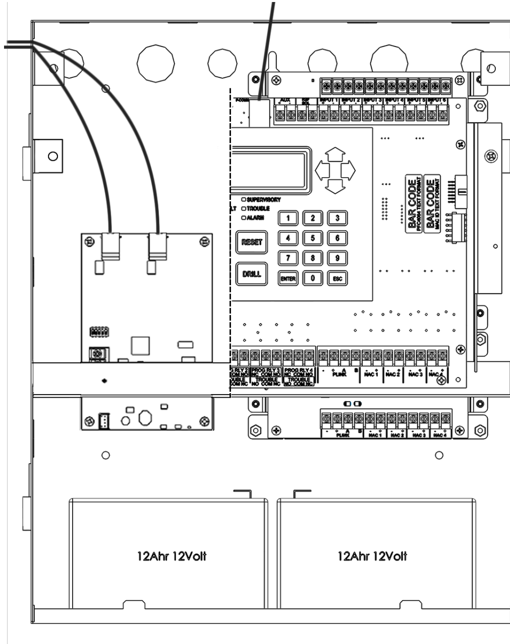
Figure 63. UD-1000 Cutaway with IP Communicator connected
