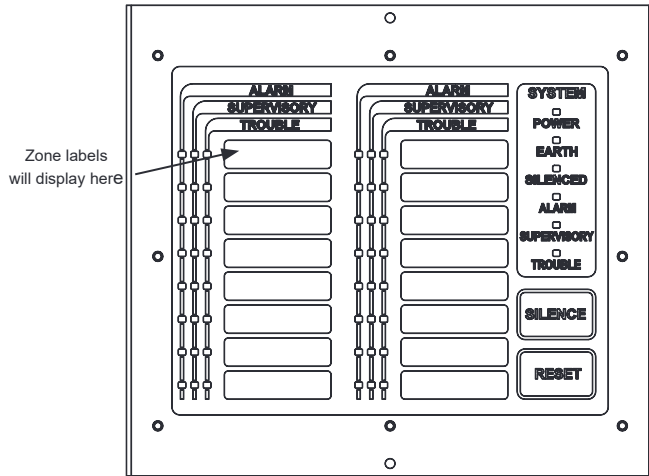
Figure 32. LED-16 Module Showing Front Panel & Board
