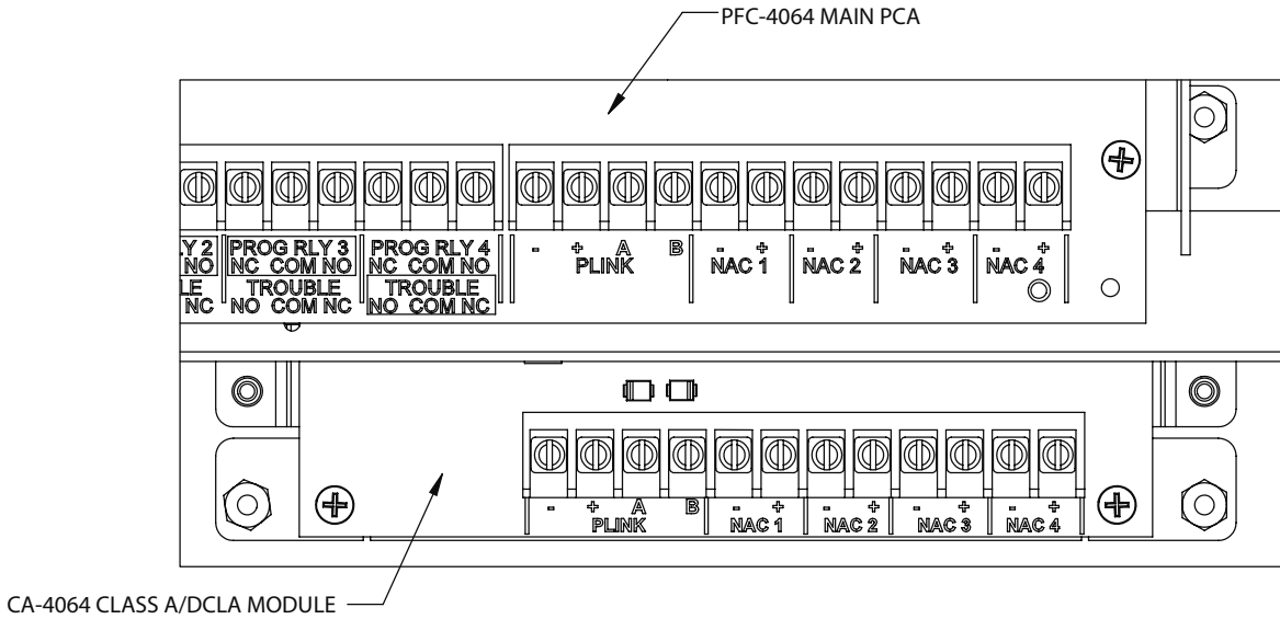
Figure 17. Example of CA-4064 Module Installed Behind Main PCA
