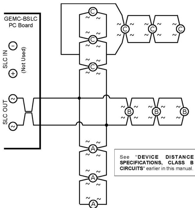
GEMC-BSLC Loop Class B wiring example
