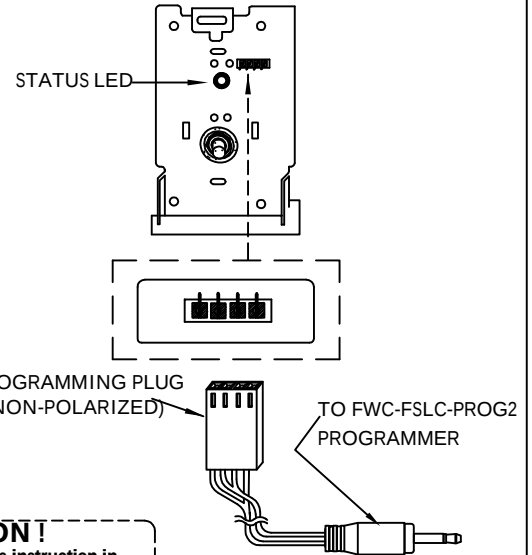
FWC-FSLC-PULL MODULE ADDRESS PROGRAMMING CONNECTION AND INDICATOR
