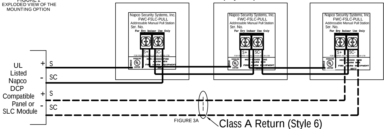
FIGURE 3 TYPICAL WIRING DIAGRAM EXAMPLE, CONNECTED TO A COMPATIBLE LISTED CONTROL PANEL
