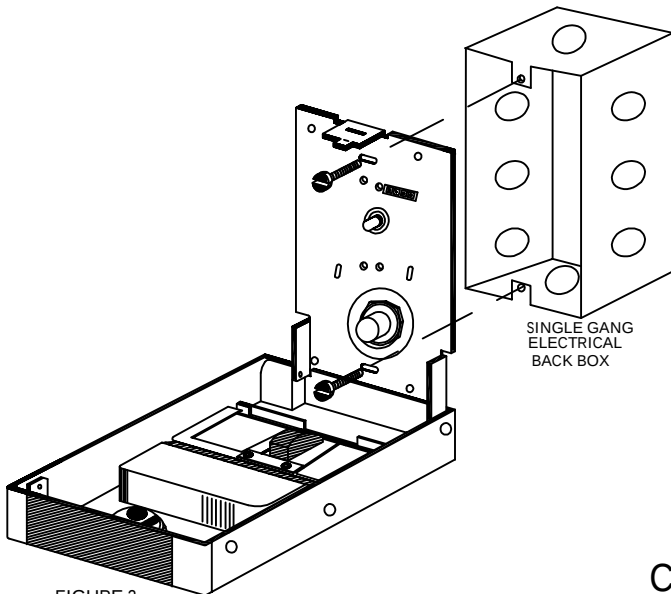
FIGURE 2 EXPLODED VIEW OF THE MOUNTING OPTION
