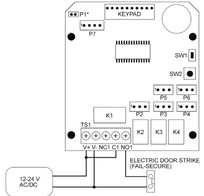
BASIC ACCESS CONTROL WITH AN ELECTRIC DOOR STRIKE
