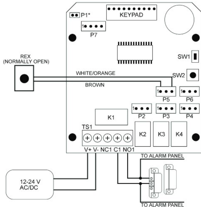
SHUNTING A NORMALLY CLOSED ZONE AND WIRING THE REX
