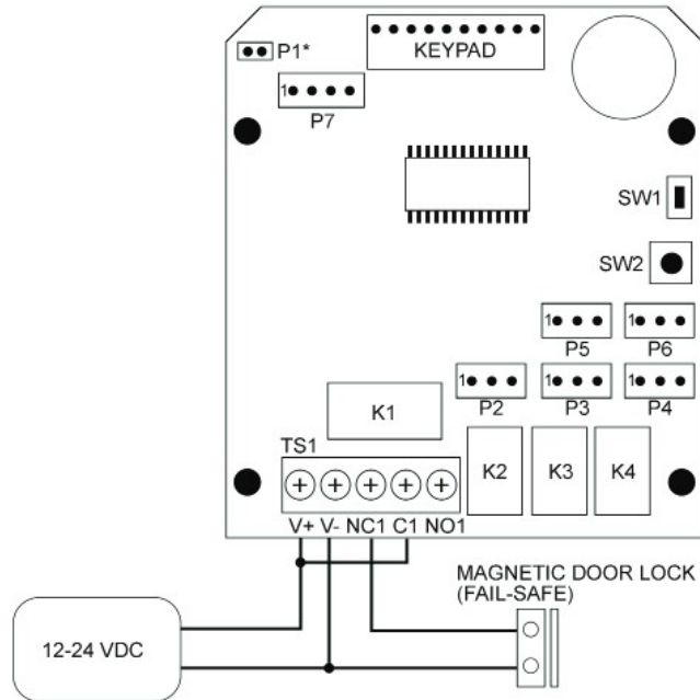
BASIC ACCESS CONTROL WITH AN ELECTROMAGNETIC DOOR LOCK
