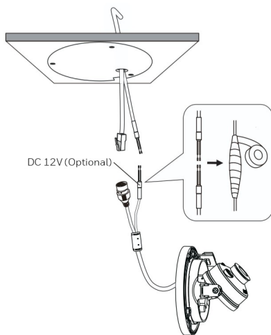
For HC35W43R3
