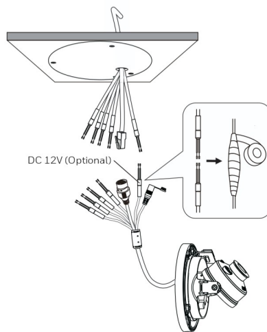
For HC35W45R3/HC35W48R3
