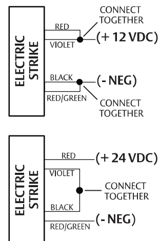
Diagram 1a: If Connector is Missing
