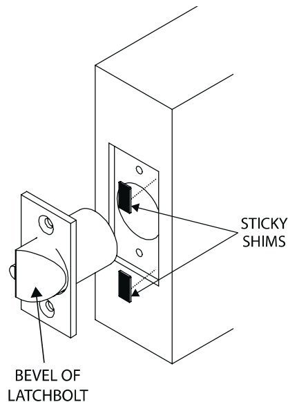
Diagram 7: Shim Installation—Door
