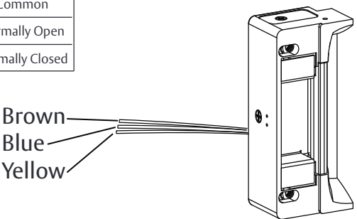
Diagram 4: Latchbolt Strike Monitor
