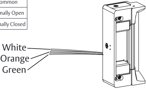
Diagram 3: Latchbolt Monitor
