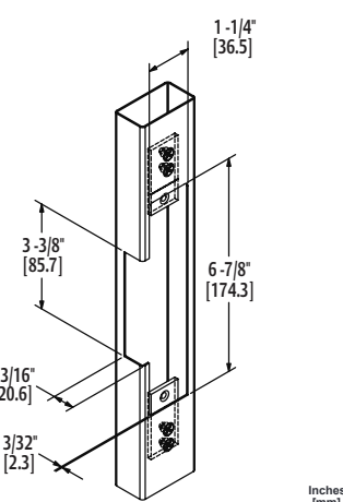
503 Faceplate Option (6-7/8" x 1-1/4"), Radius Corners and Flat Faceplate Used with cylindrical locksets or spring latches in aluminum frames
