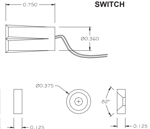
SWITCH
