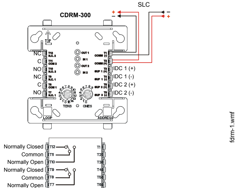
Figure 8.1 CDRM-300 Wiring Connections
