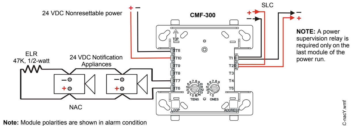
Figure 6.2 NFPA Style Y Notification Appliance Circuit
