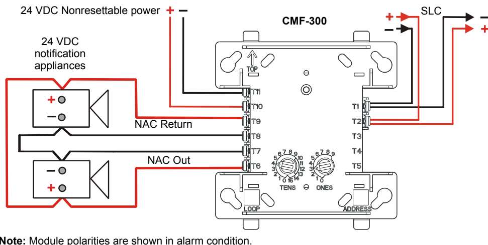
Figure 6.3 NFPA Style Z Notification Appliance Circuit
