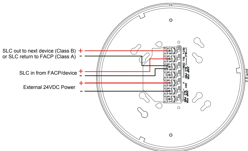
Figure 9.7 W-GATE Powered by a Regulated, External Source
