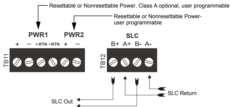
Figure 2.12 ES-200X Terminal Blocks
