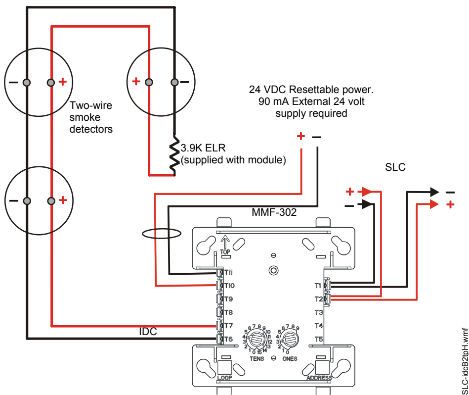
Figure 5.15 Typical Style B IDC Wiring with an MMF-302
