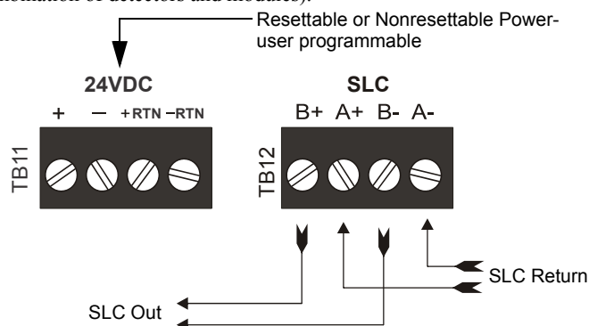
Figure 2.11 ES-50X Terminal Block
