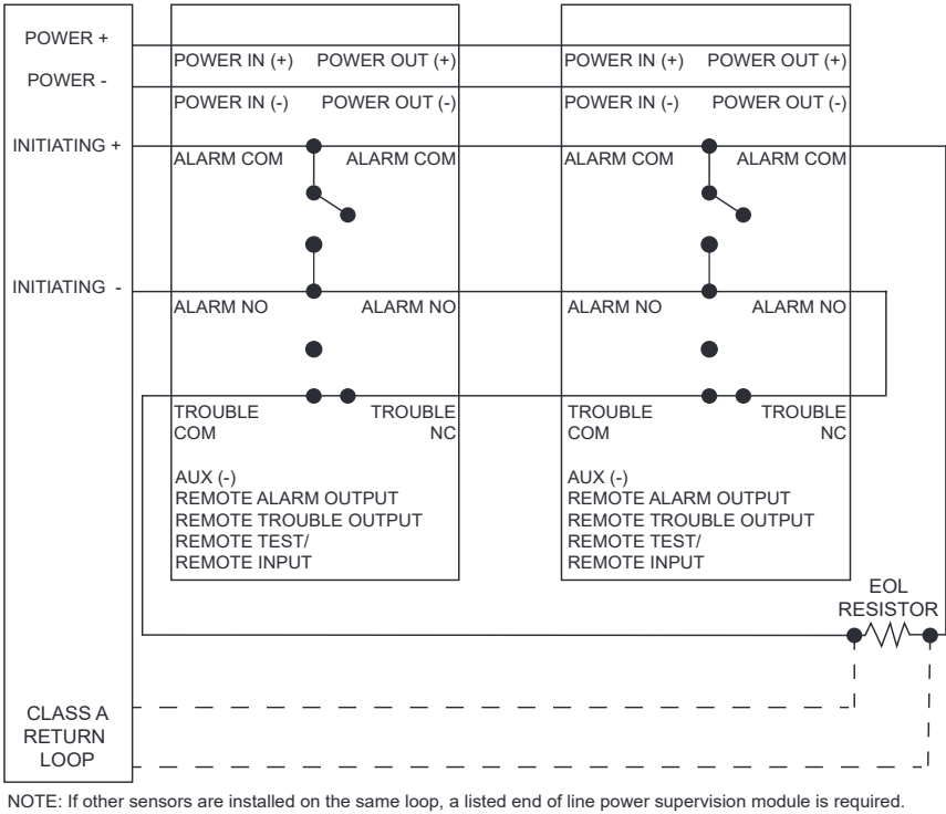
Figure 11-2: Wiring Diagram
