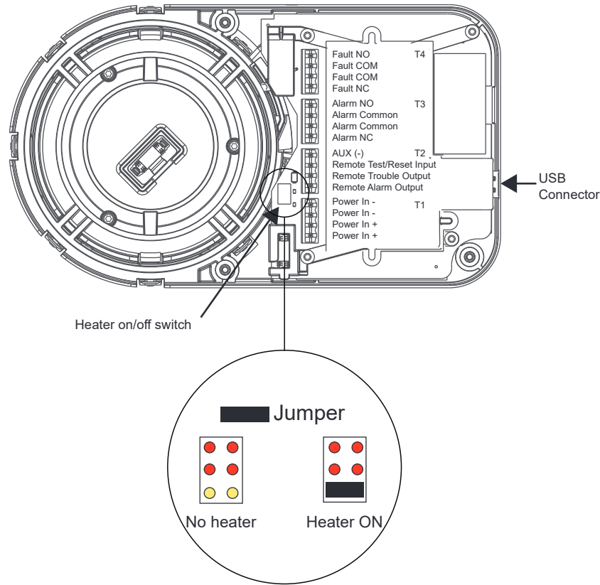
Figure 11-3: Wiring Connections at Detector
