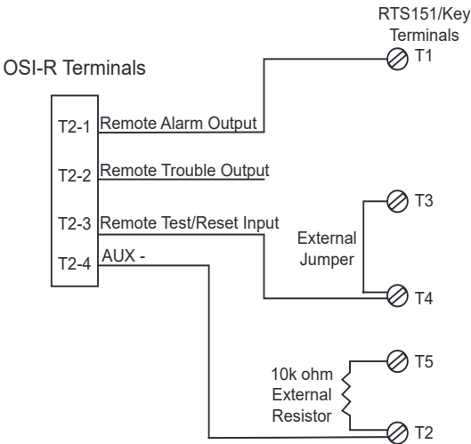
Figure 11-4: Wiring Diagram (RTS451 or RTS151)
