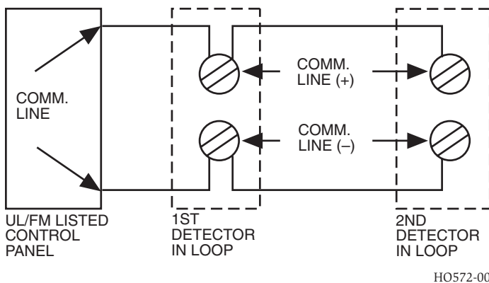
FIGURE 6. SYSTEM WIRING DIAGRAM FOR D365PL
