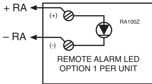
FIGURE 8. WIRING DIAGRAM FOR D365PL TO RA100Z
