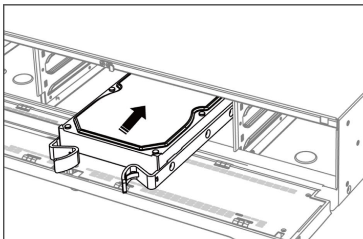
Figure 1-9 Insert HDD
