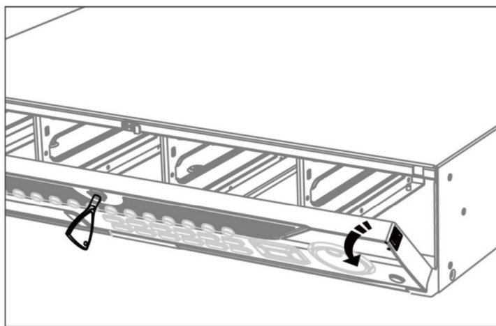
Figure 1-8 Open Front Panel
