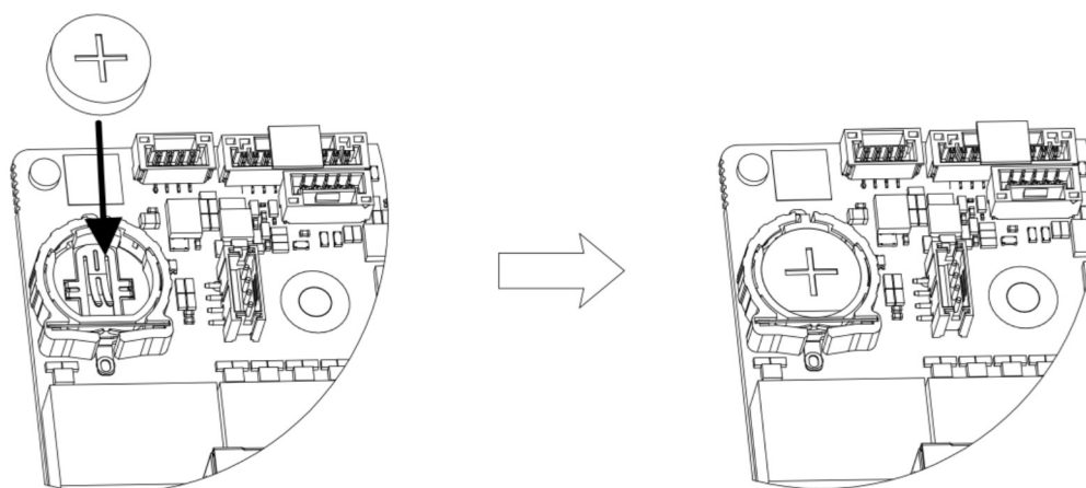
Figure 1-2 Replace Battery
