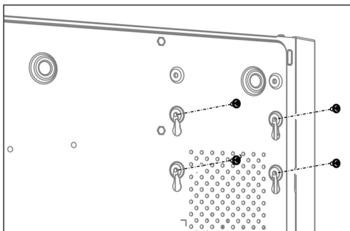
Figure 1-12 Fix HDD to Device Bottom
