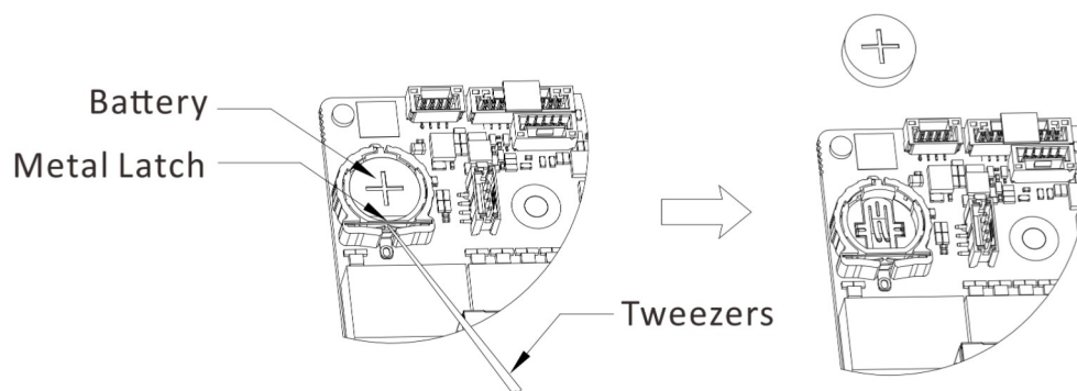
Figure 1-1 Remove Battery
