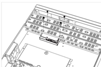
Figure 1-5 Fix HDD
