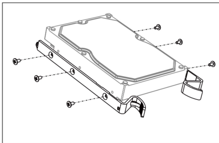
Figure 1-7 Fix Mounting Ears to HDD
