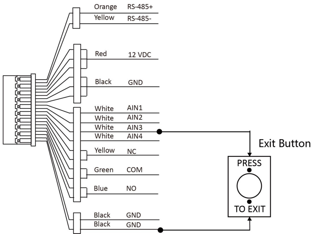
Figure 2-4 Exit Botton Wiring
