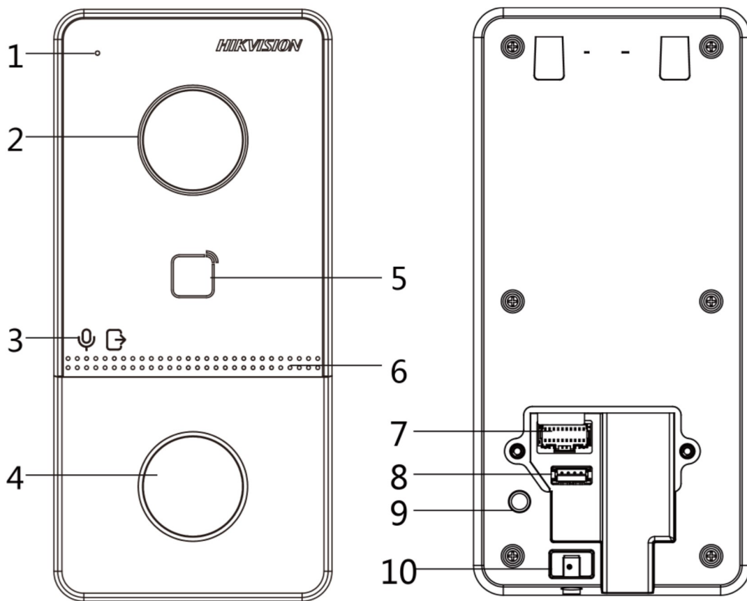
Figure 1-1 Front Panel and Rear Panel
