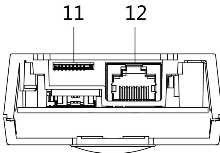
Figure 1-2 Bottom Panel
