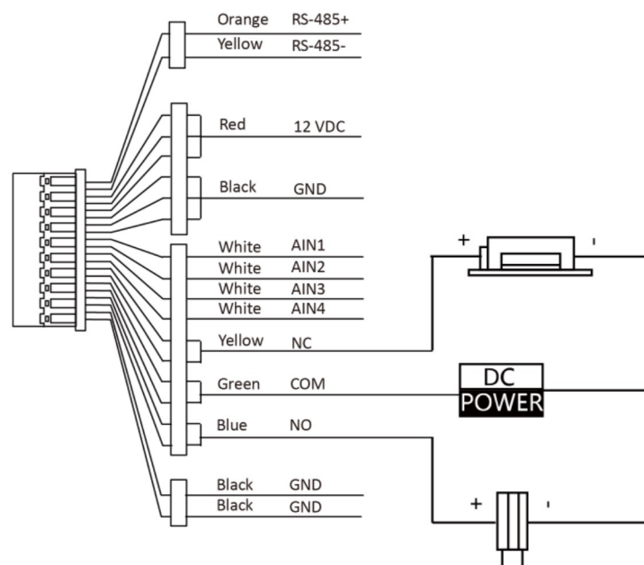
Figure 2-2 Door Lock Wiring
