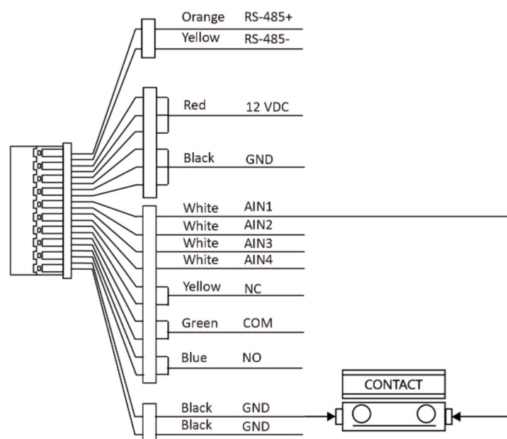
Figure 2-3 Door Contact Wiring
