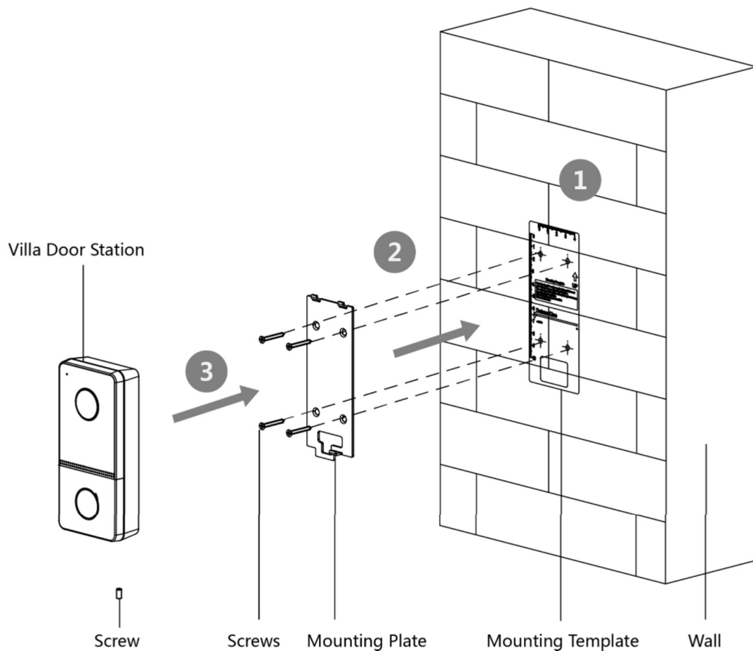
Figure 3-4 Surface Mounting without Protective Shield
