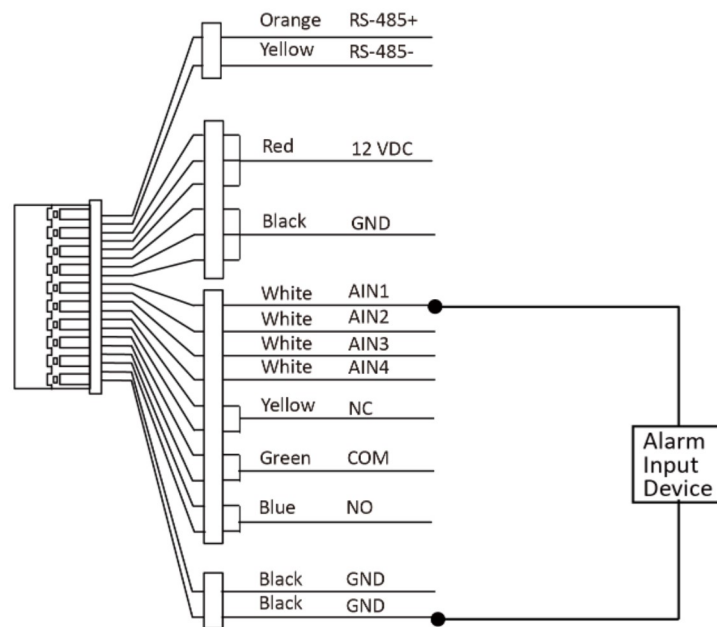
Figure 2-5 Alarm Input Device Wiring
