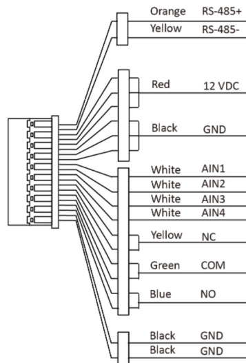
Figure 2-1 Terminal Description
