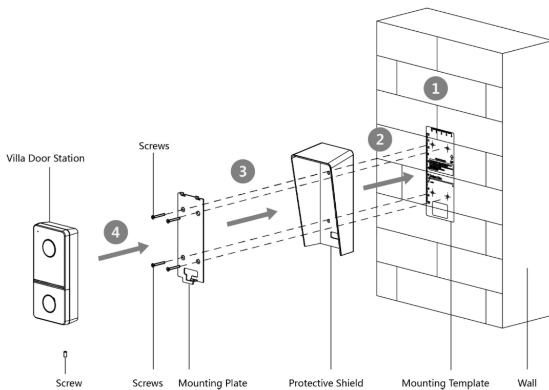
Figure 3-6 Surface Mounting with Protective Shield
