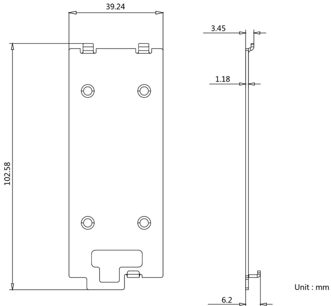
Figure 3-1 Accessory Introduction
