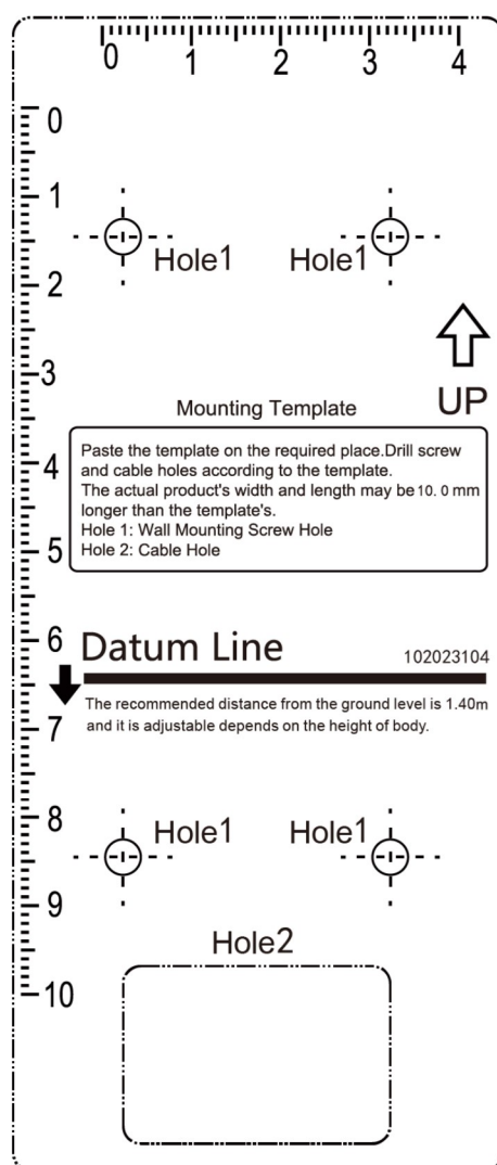
Figure 3-5 Mounting Template
