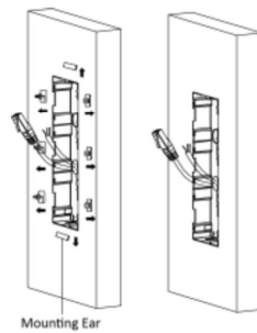
Figure 3-41 Remove the Mounting Ears
