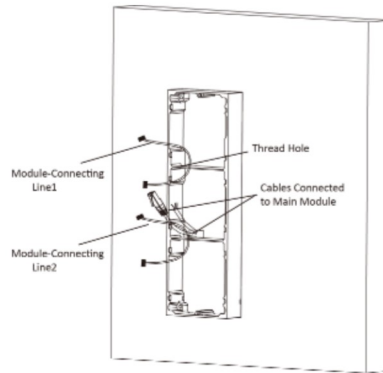
Figure 3-33 Placement of Lines
