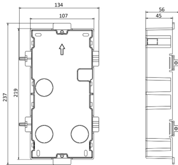
Figure 3-22 Gang Box
