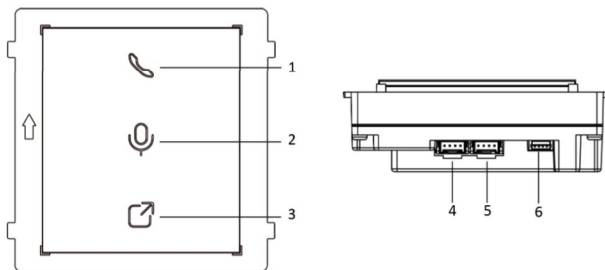
Figure 1-5 Indicator Module
