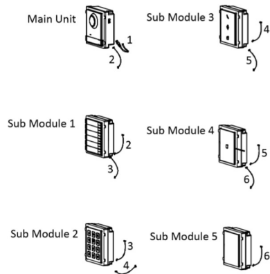
Figure 3-61 Cables Connection
