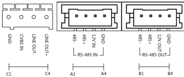
Figure 2-4 Touch-Display Module
