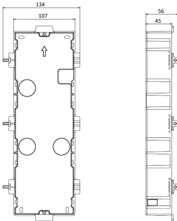
Figure 3-37 Gang Box
