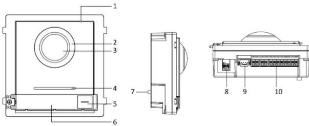
Figure 1-2 Two-Wire Main Unit
