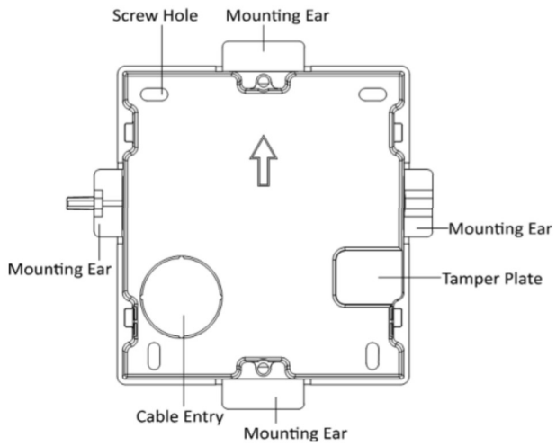
Figure 3-8 Gang Box
