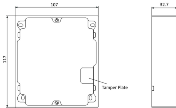
Figure 3-2 Mounting Frame
