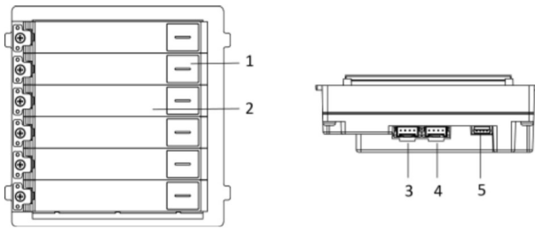
Figure 1-3 Nametag Module Appearance
