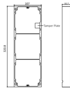
Figure 3-44 Mounting Frame
