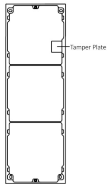
Figure 3-32 Mounting Frame
