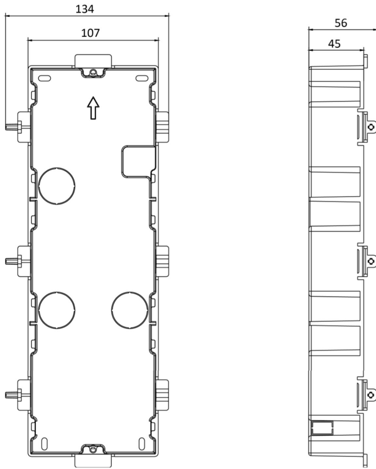
Figure 3-53 Gang Box
