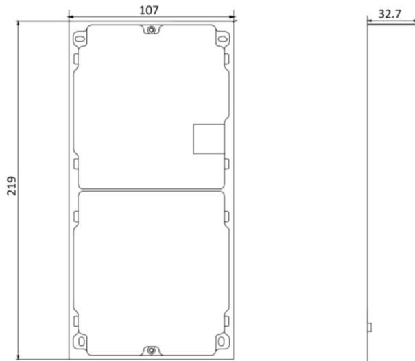
Figure 3-15 Mounting Frame
