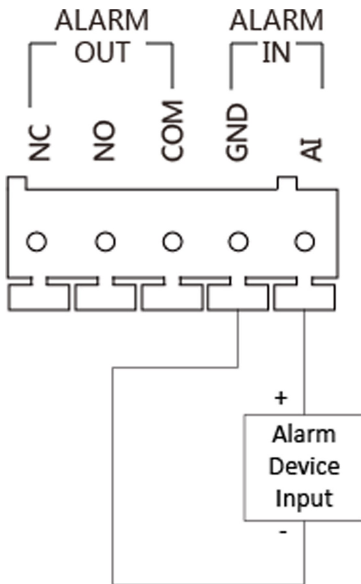
Figure 2-5 Alarm Device Input Wiring
