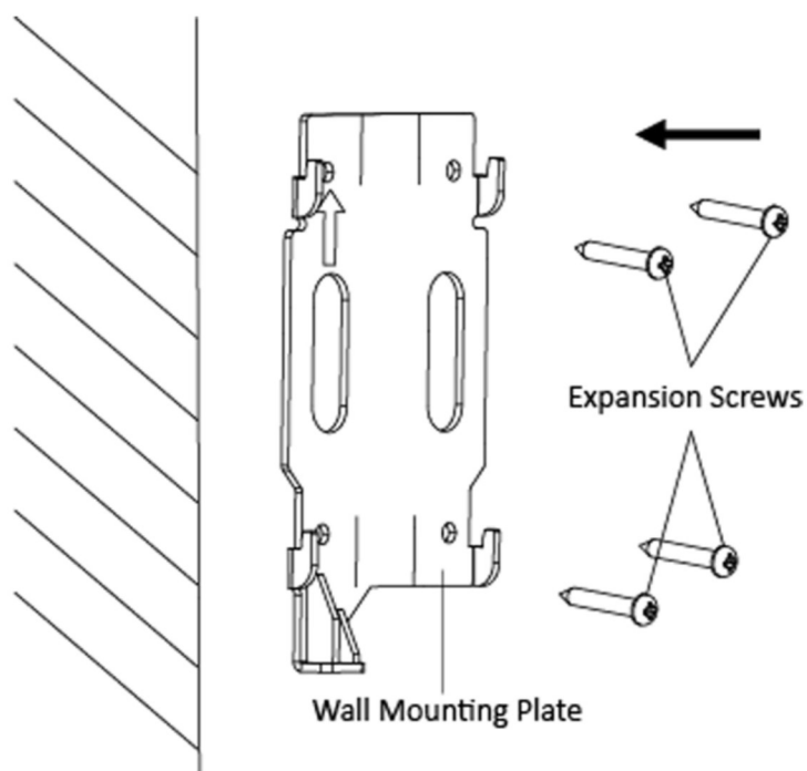
Figure 3-2 Install the Plate
