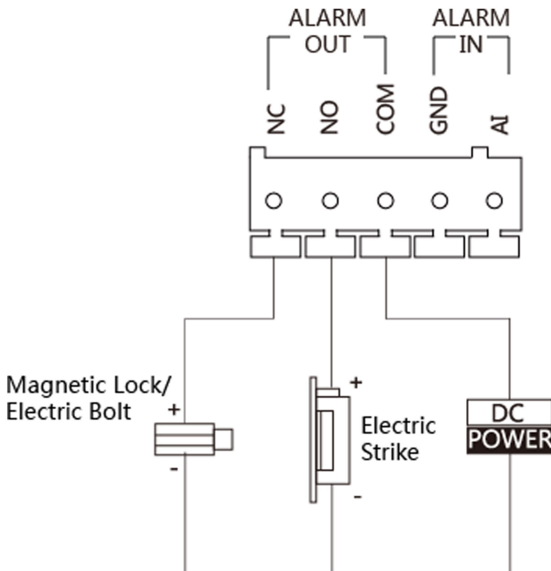
Figure 2-2 Door Lock Wiring
