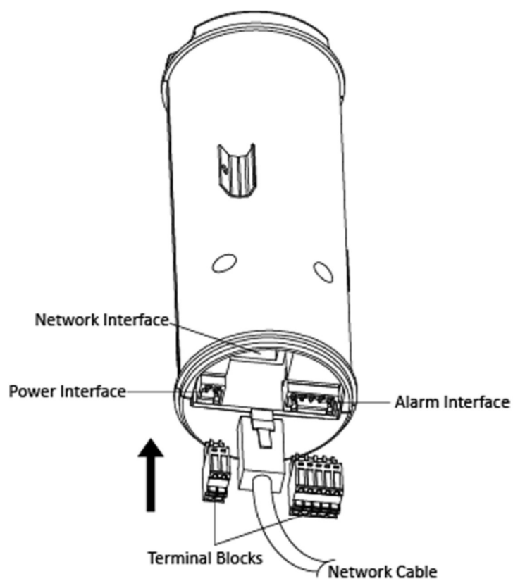
Figure 3-3 Insert Terminals and Network Cable
