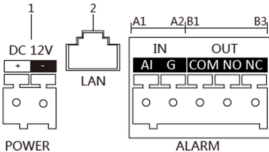
Figure 2-1 Terminals Description
