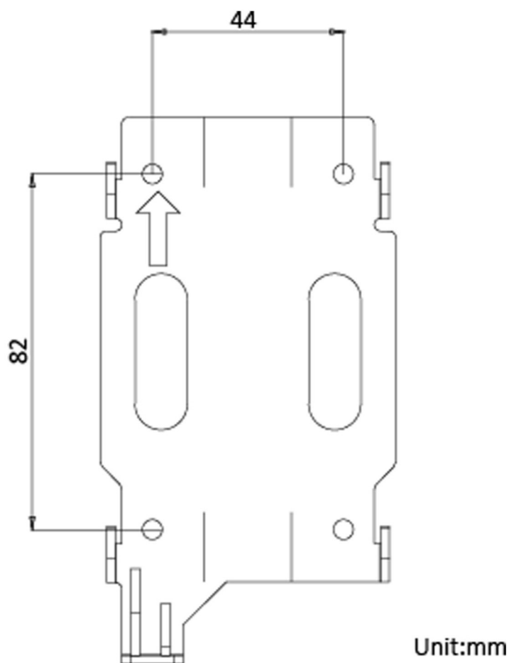
Figure 3-1 Wall Mounting Plate
