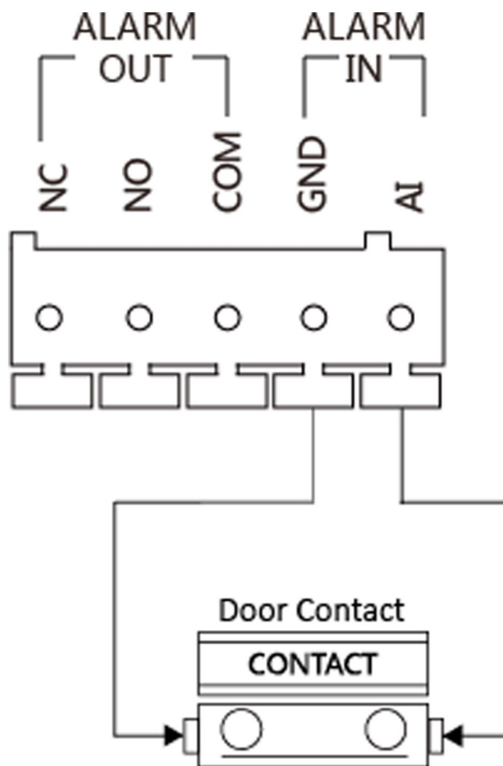
Figure 2-3 Door Contact Wiring
