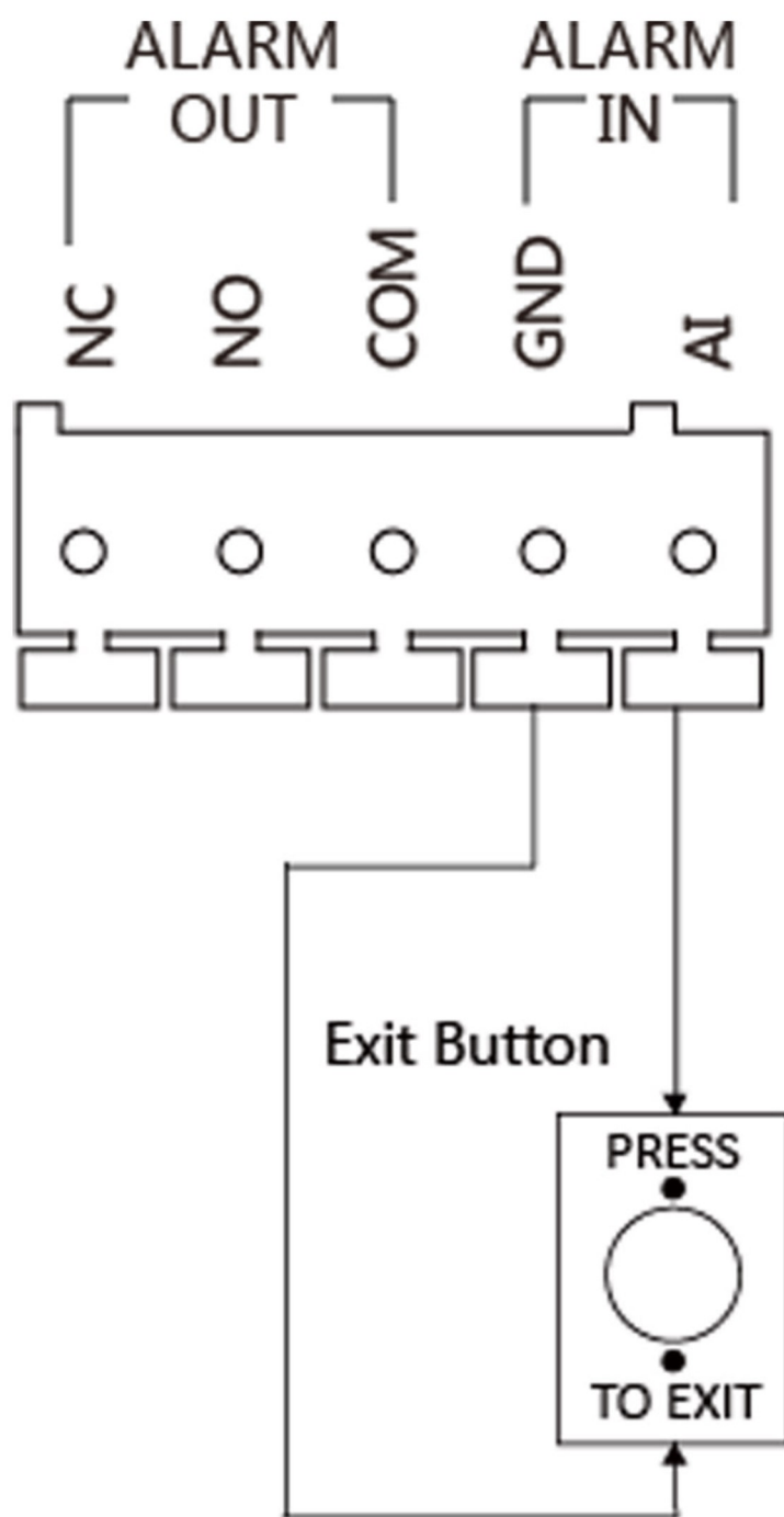
Figure 2-4 Exit Button Wiring
