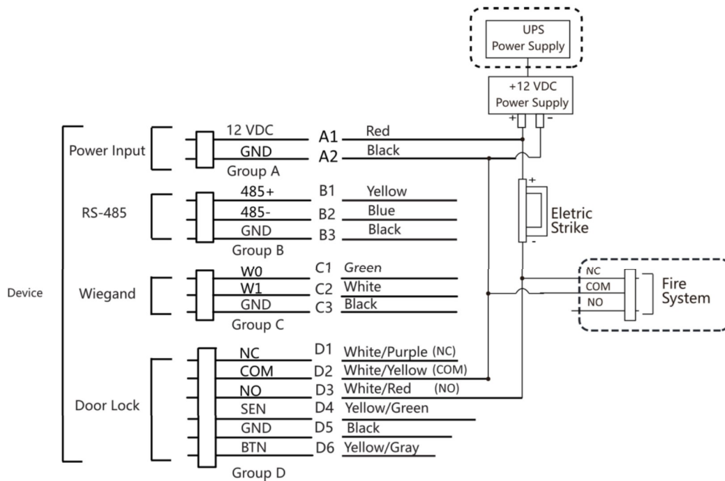
Figure 4-7 Device Wiring
