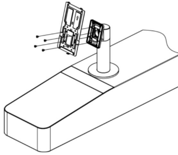
Figure 3-19 Fix Mounting Plate
