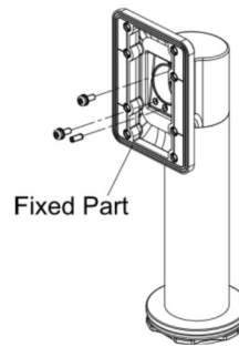
Figure 3-12 Rotate Fixed Part
