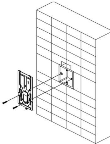
Figure 3-2 Install Mounting Plate
