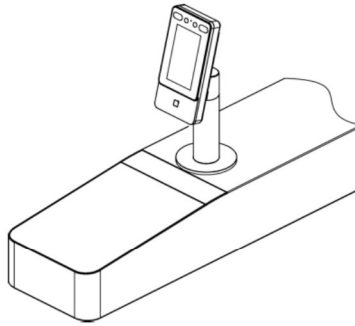
Figure 3-20 Fix Mounting Plate
