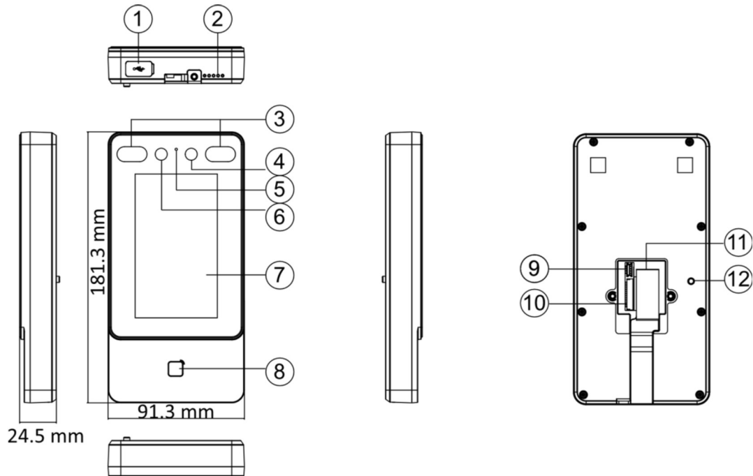
Figure 2-2 Without Fingerprint Module
