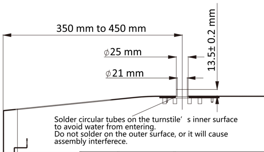
Figure 3-17 Solder Tubes
