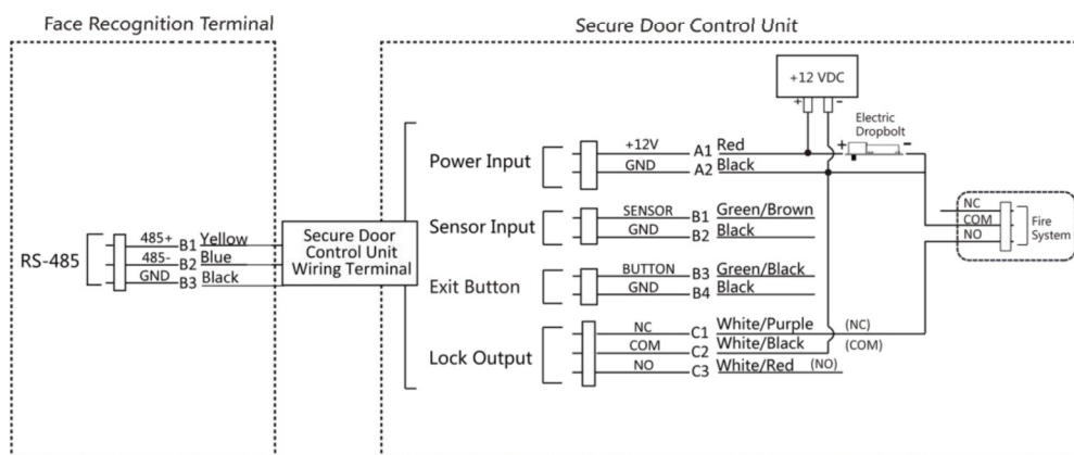
Figure 4-6 Wiring Secure Door Control Unit
