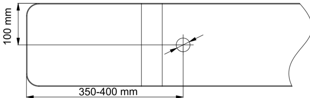
Figure 3-10 Drill Holes on Turnstile
