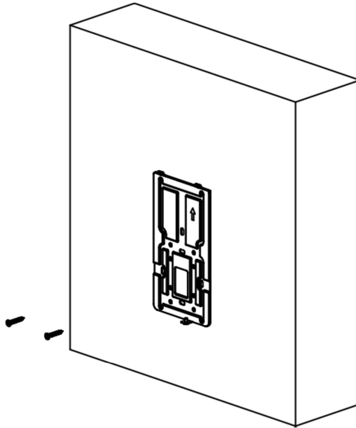
Figure 3-6 Install Mounting Plate
