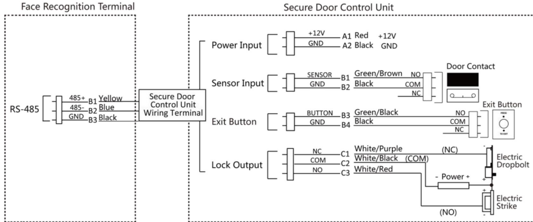
Figure 4-2 Secure Door Control Unit Wiring
