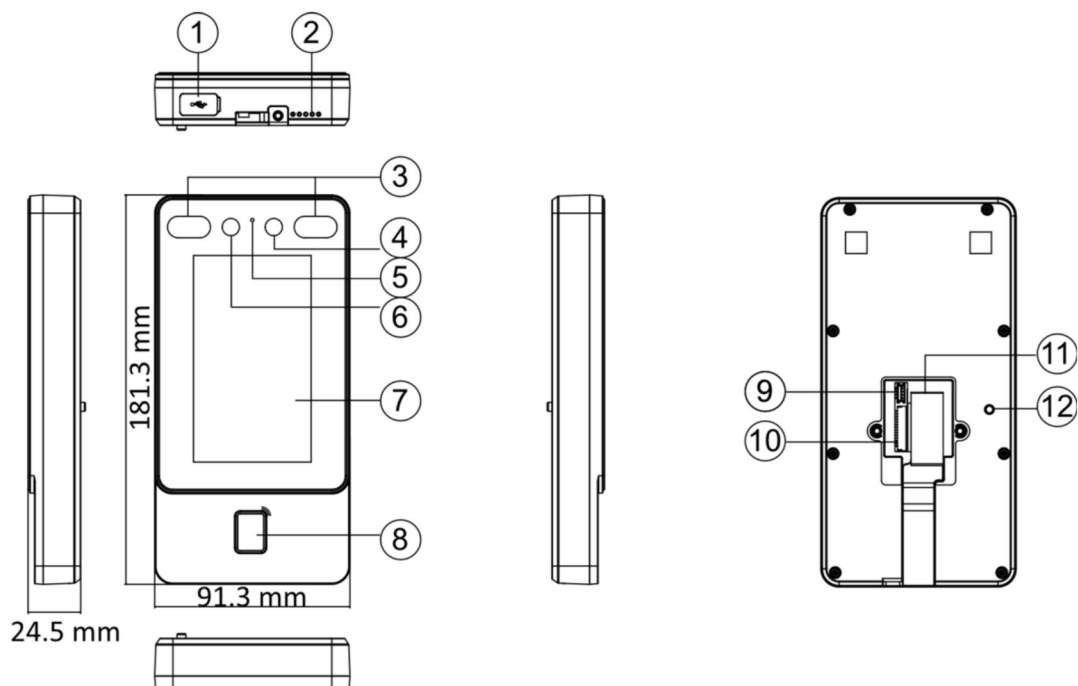
Figure 2-1 With Fingerprint Module
