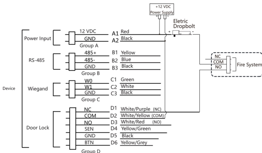
Figure 4-5 Wiring Device
