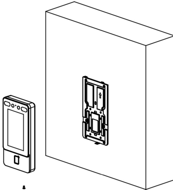
Figure 3-8 Hang Device
