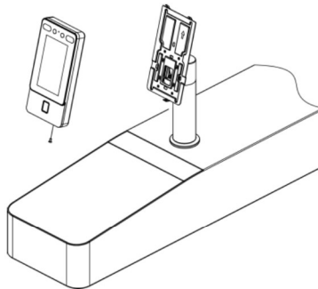
Figure 3-15 Fix the Device
