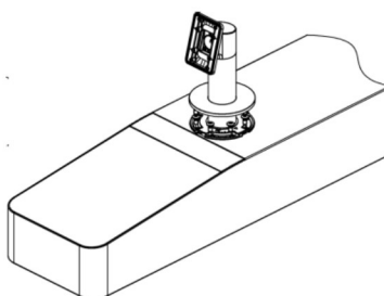
Figure 3-18 Install Base
