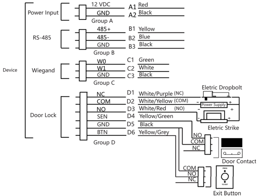
Figure 4-1 Device Wiring
