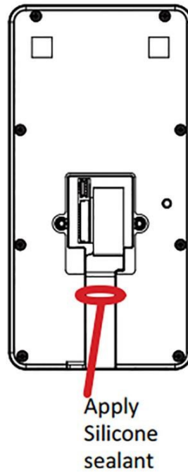
Figure 3-3 Apply Silicone Sealant
