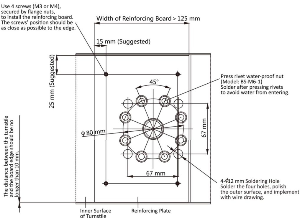
Figure 3-16 Drill Holes on Turnstile
