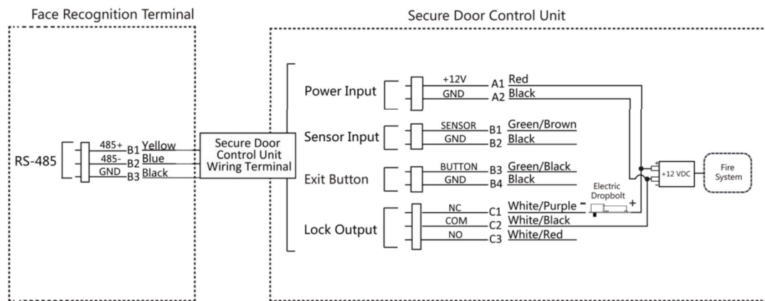
Figure 4-4 Wire Secure Door Control Unit
