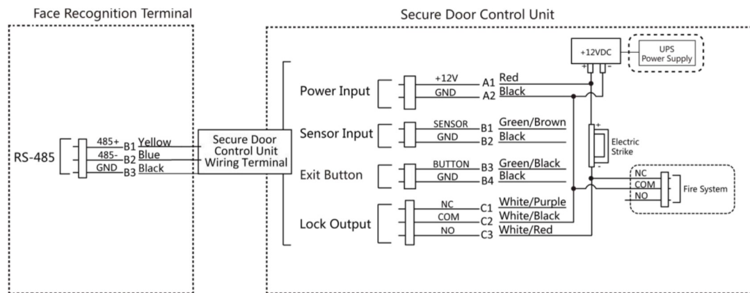
Figure 4-8 Wiring Diagram
