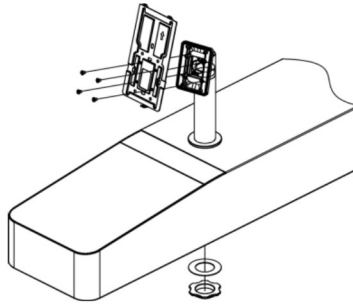
Figure 3-14 Secure Mounting Template
