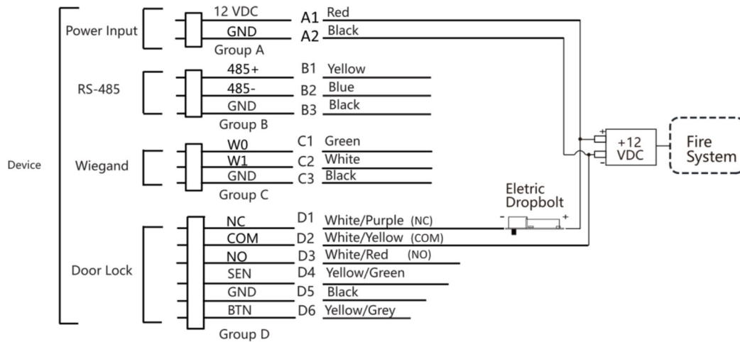
Figure 4-3 Wire Device
