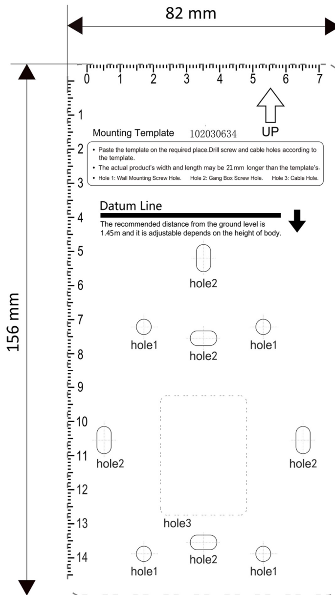
Figure 3-5 Mounting Template
