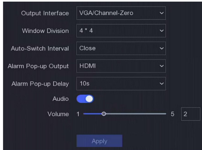
Figure 6-1 Live View-General
