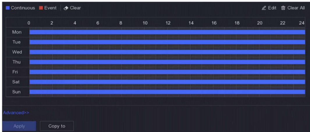
Figure 6-23 Recording Schedule
