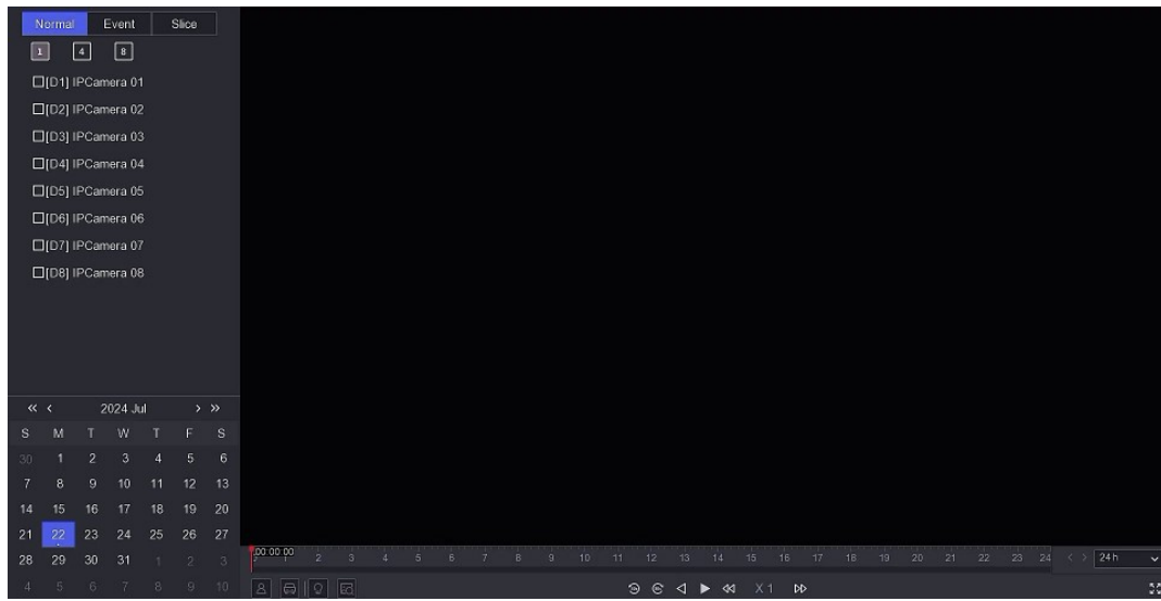
Figure 3-1 Playback
