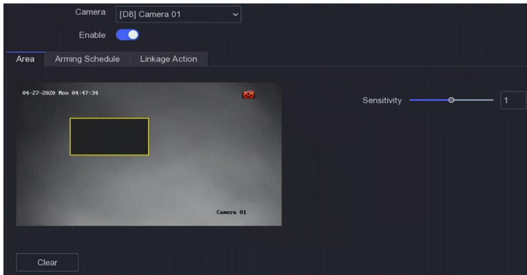
Figure 6-13 Video Tampering
