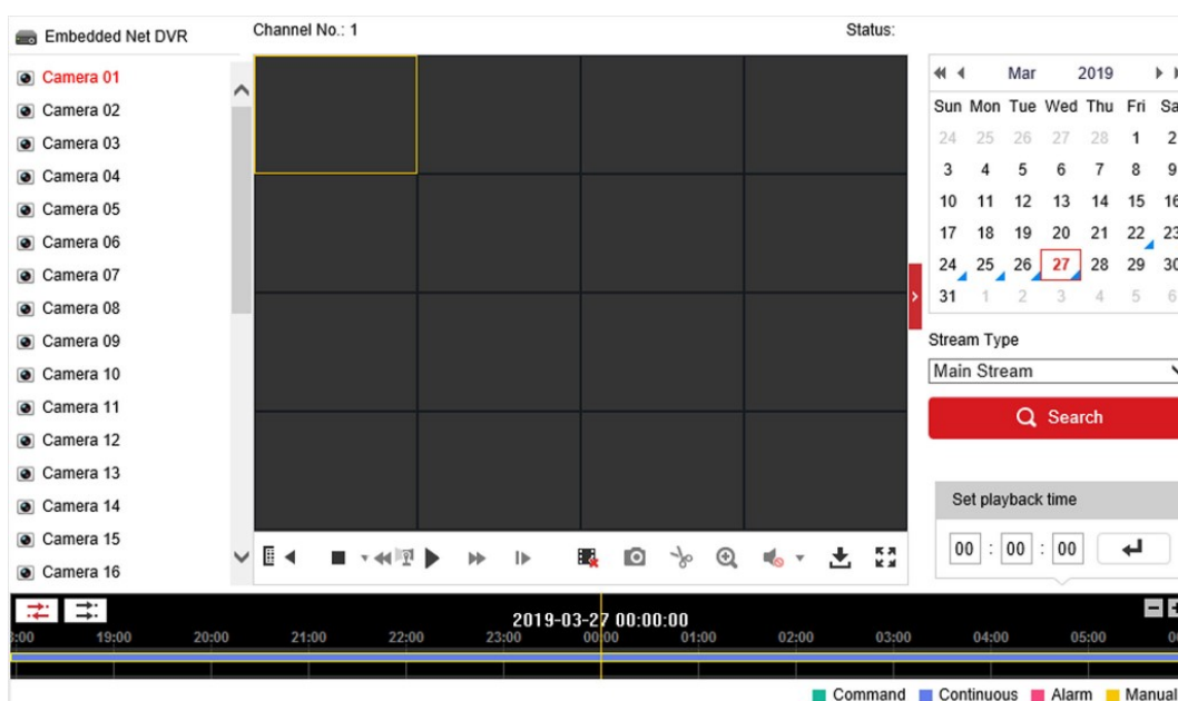
Figure 9-3 Playback
