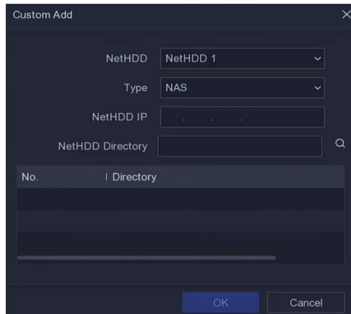
Figure 5-9 Add NetHDD
