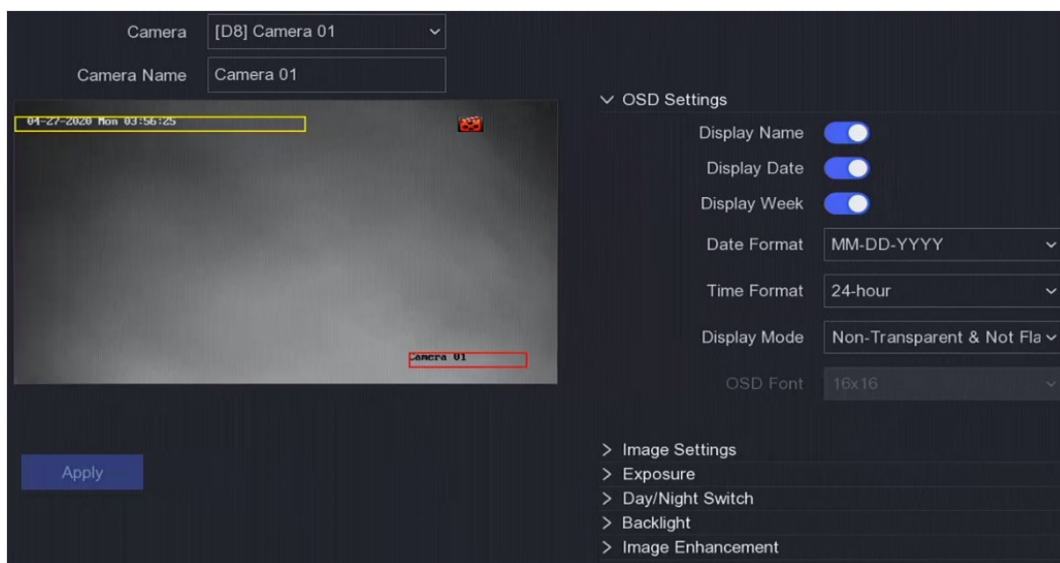
Figure 6-11 OSD
