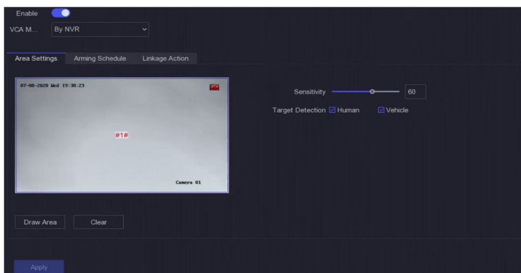
Figure 5-7 Motion Detection
