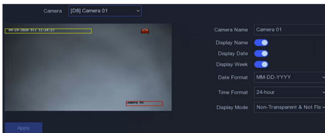
Figure 5-6 OSD
