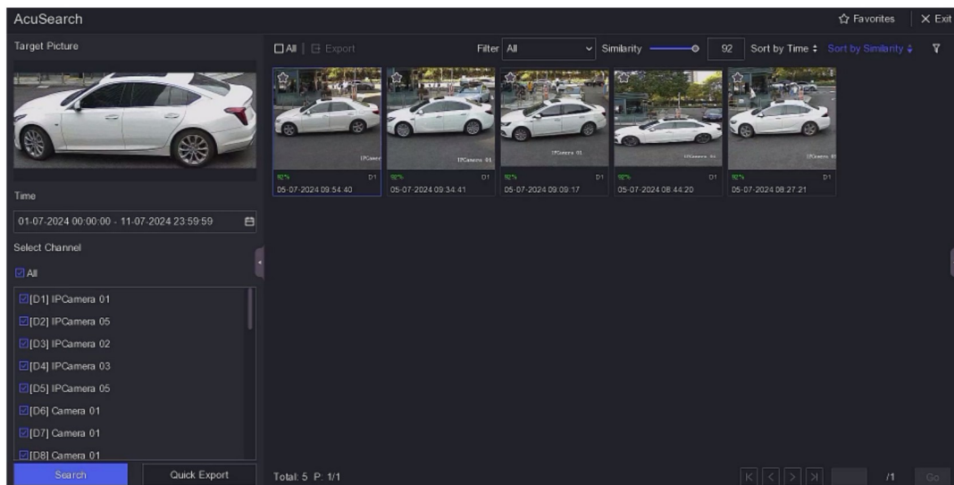
Figure 3-5 AcuSearch
