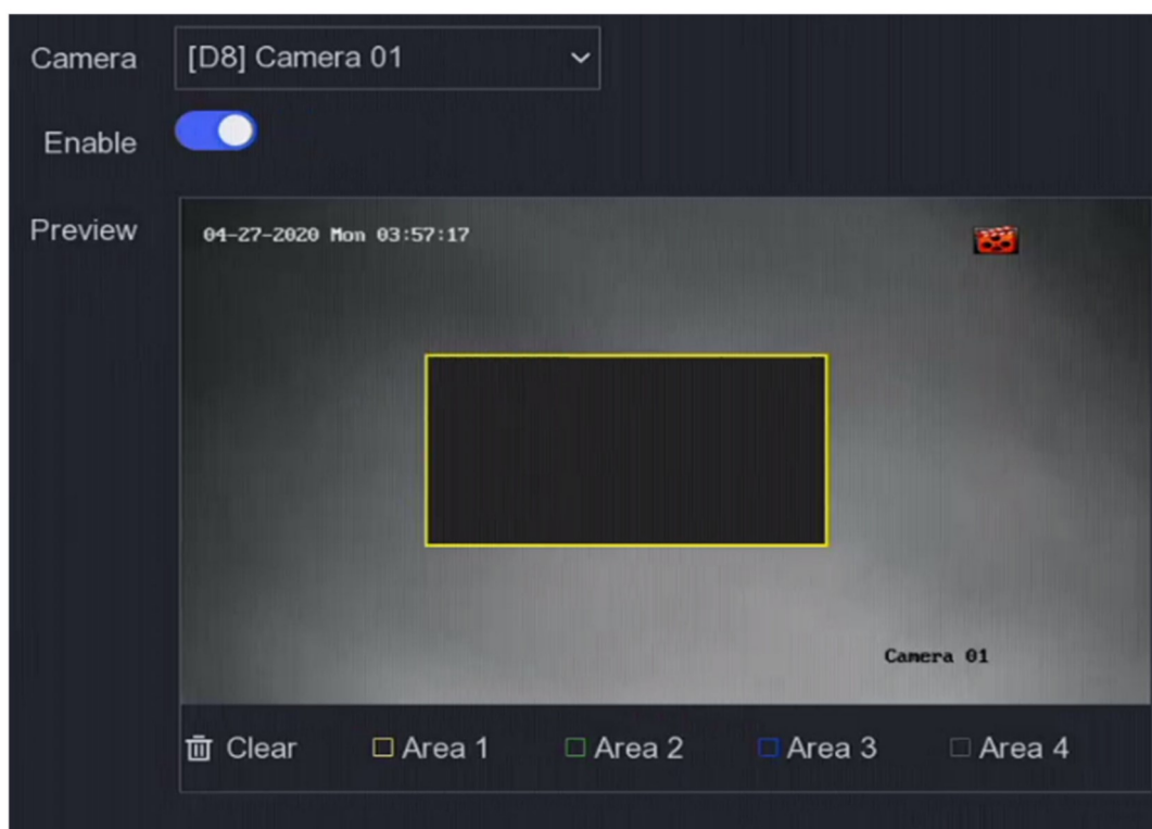
Figure 6-12 Privacy Mask
