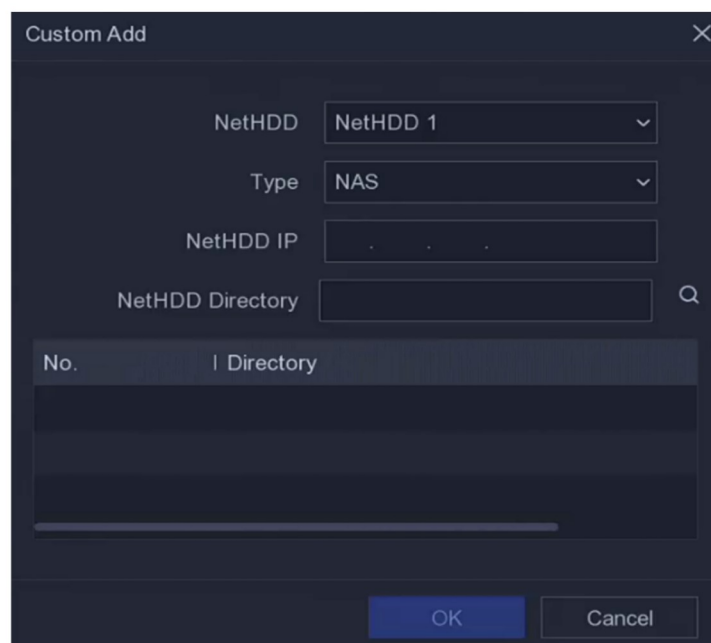
Figure 6-24 Add NetHDD
