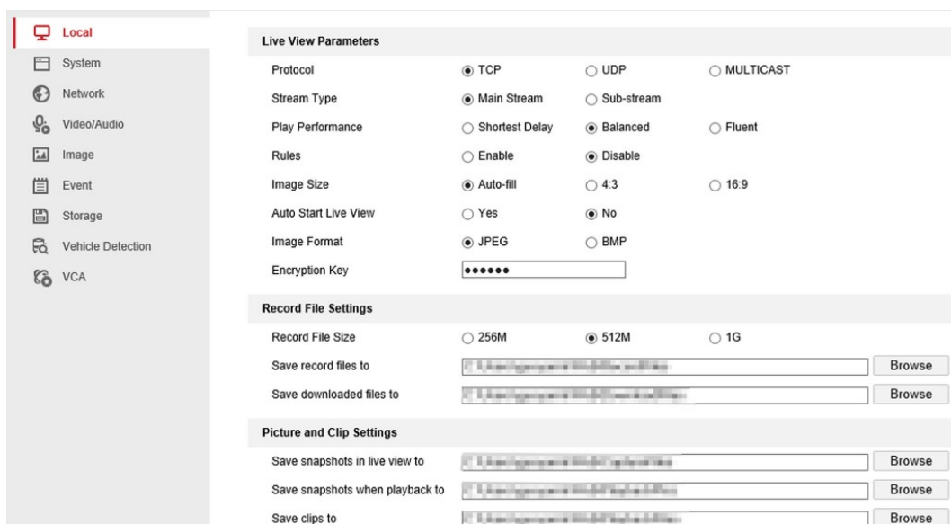
Figure 9-4 Configuration
