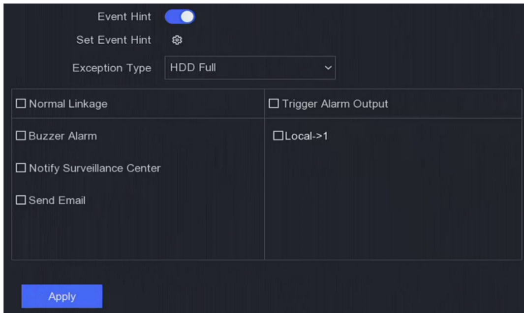
Figure 6-18 Exceptions
