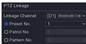
Figure 6-22 PTZ Linkage
