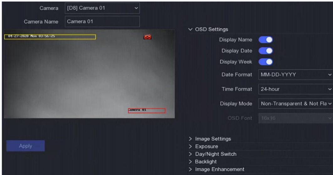
Figure 6-12 OSD
