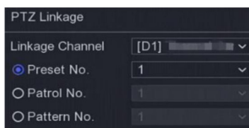
Figure 6-21 PTZ Linkage
