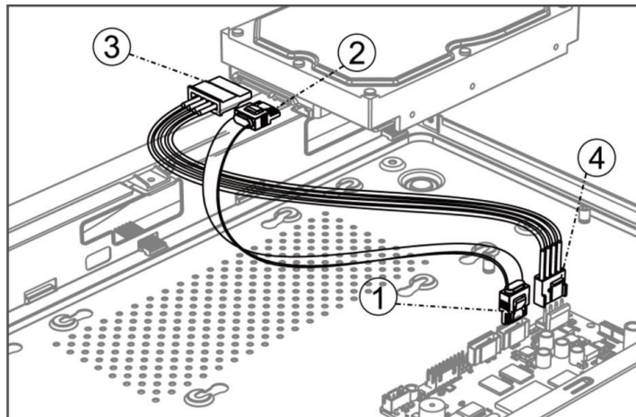
Figure 1-11 Connect Cables
