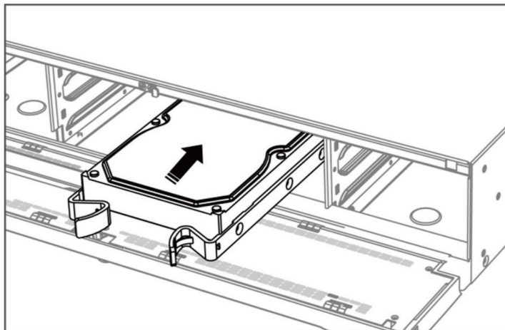
Figure 1-7 Insert HDD
