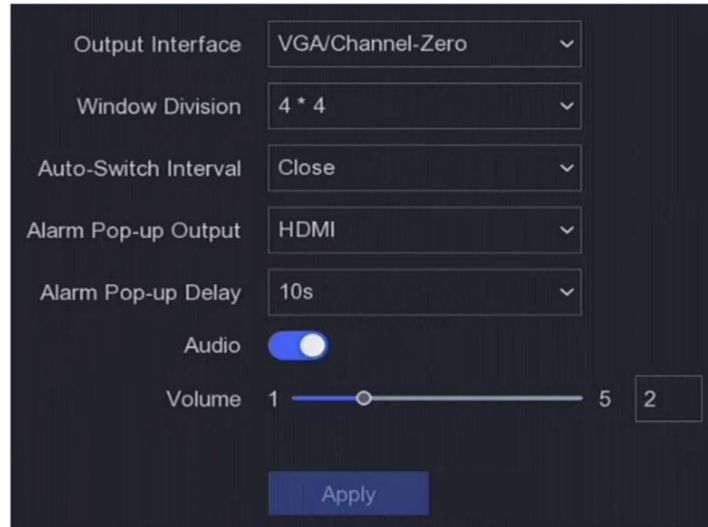
Figure 6-1 Live View-General
