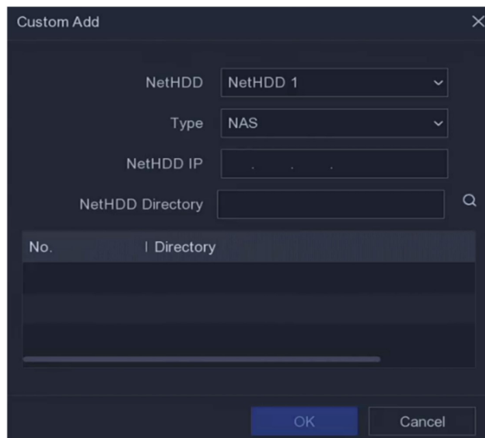
Figure 6-23 Add NetHDD
