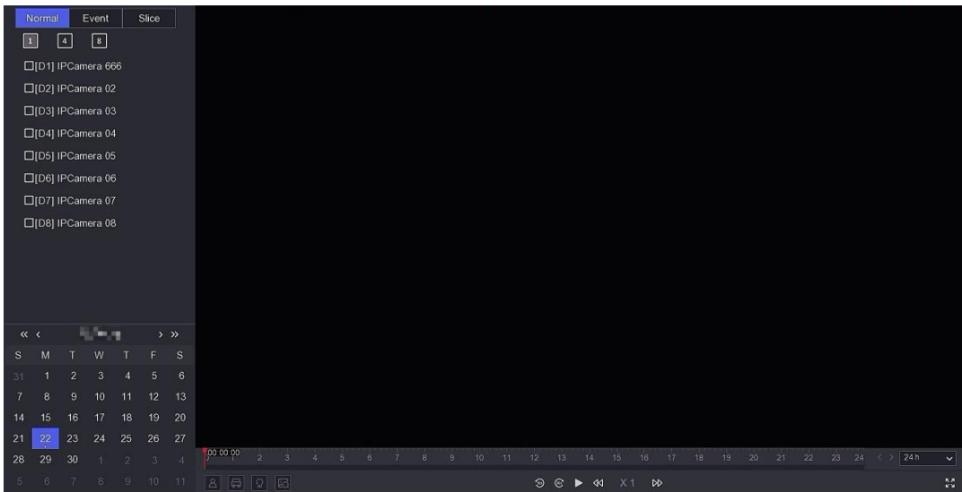
Figure 3-1 Playback
