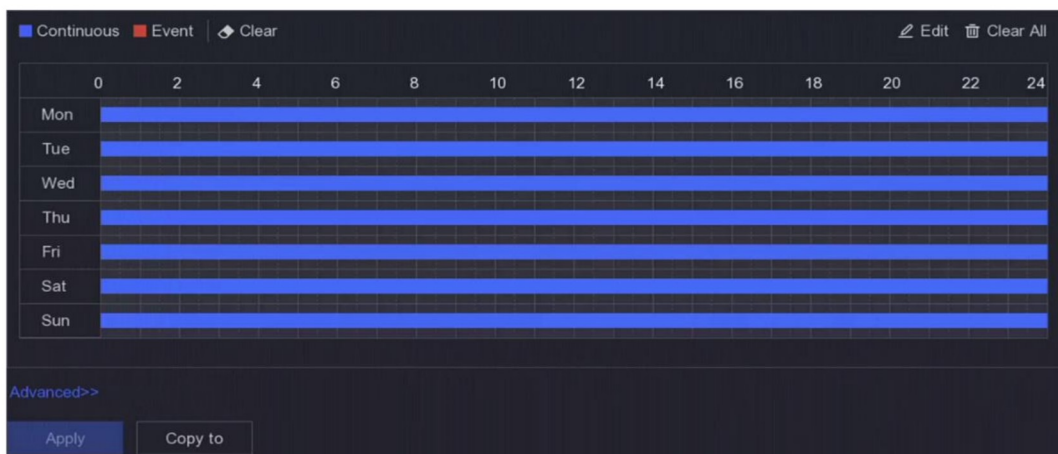
Figure 6-22 Recording Schedule
