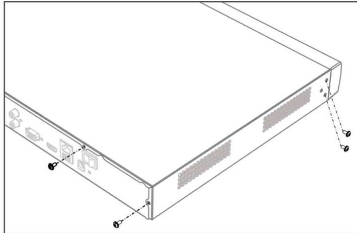
Figure 1-10 Remove Cover
