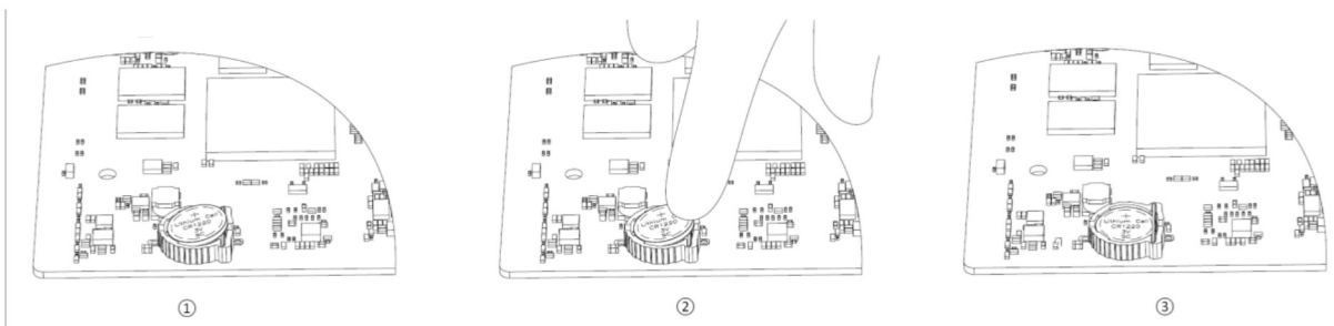
Figure 1-2 Replace Battery
