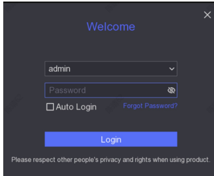
Figure 1-3 Login Interface
