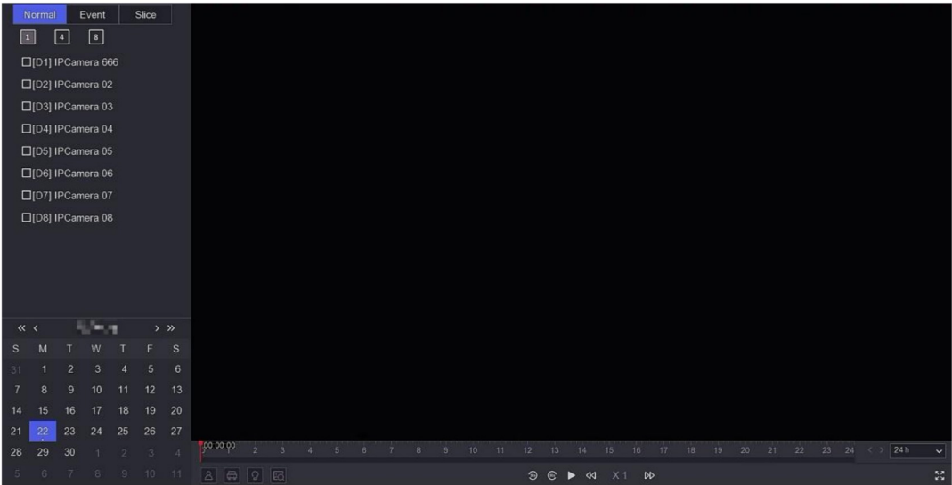
Figure 3-3 Playback
