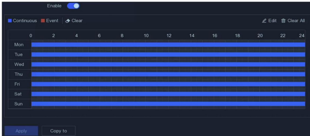
Figure 5-10 Recording Schedule
