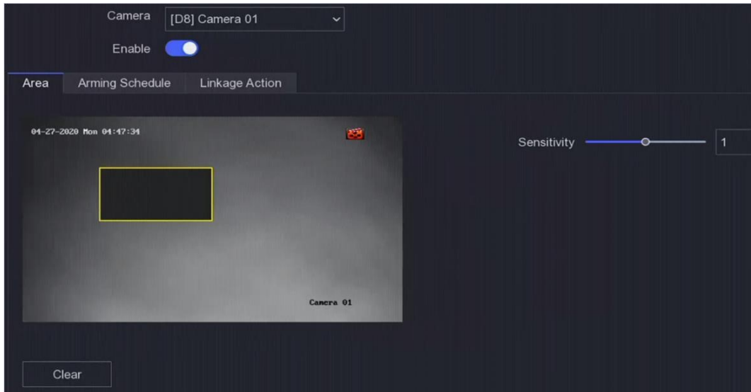
Figure 6-14 Video Tampering
