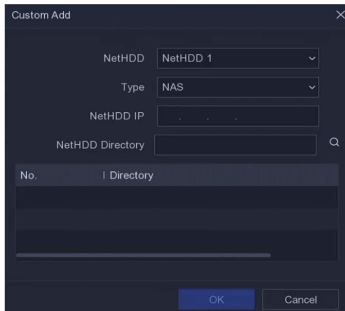
Figure 5-9 Add NetHDD
