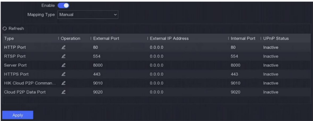
Figure 6-4 NAT
