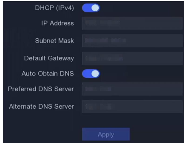
Figure 5-2 Network
