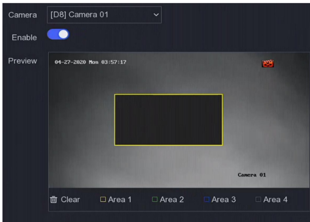
Figure 6-13 Privacy Mask
