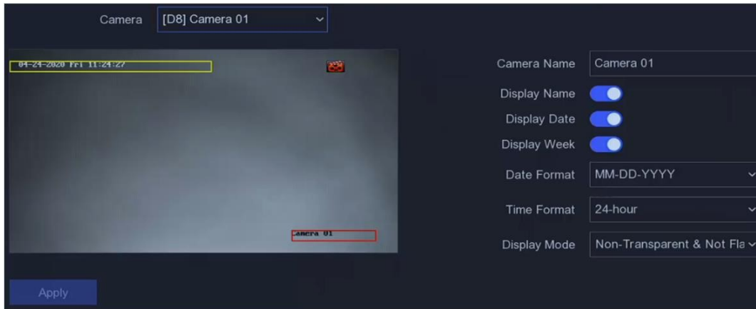
Figure 5-7 OSD
