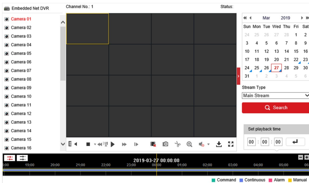
Figure 9-3 Playback
