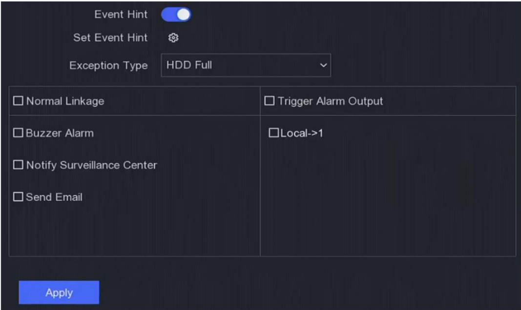
Figure 6-19 Exceptions
