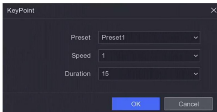
Figure 2-4 Patrol Settings
