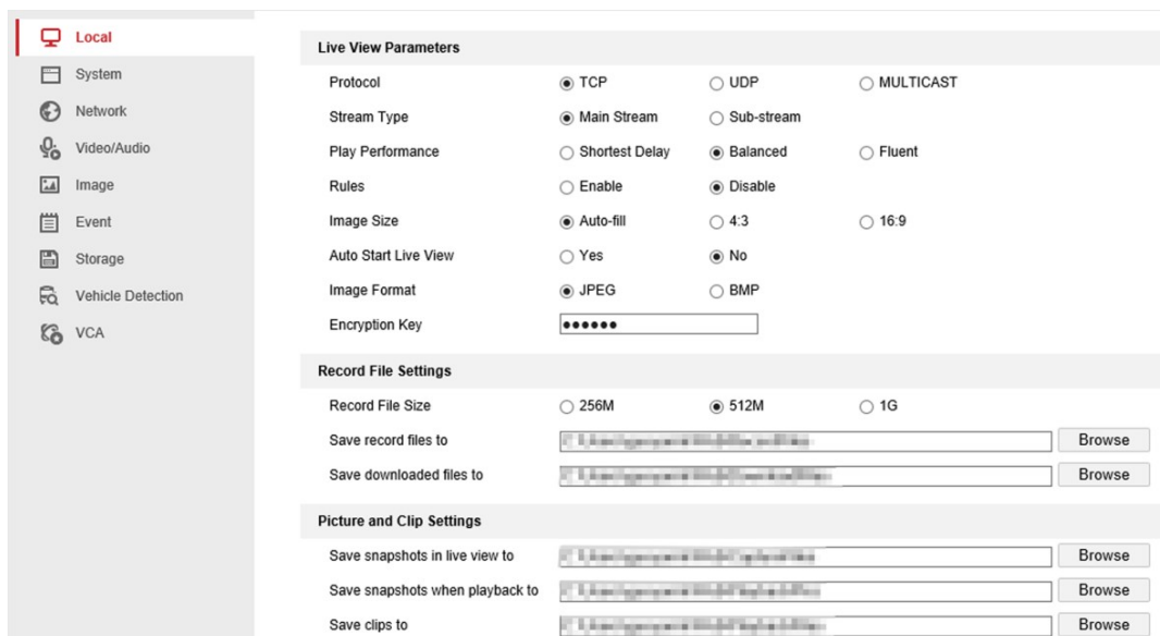
Figure 9-4 Configuration
