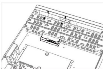
Figure 1-3 Fix HDD
