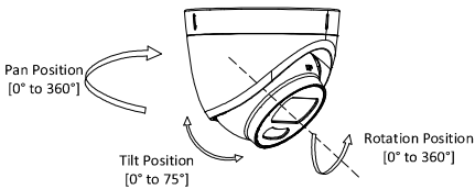
Figure 2-16 3-Axis Adjustment
