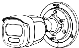
Figure 2-5 Attach the Camera on the Junction Box's Cover
