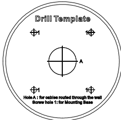
Figure 2-17 Drill Template
