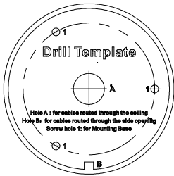
Figure 2-13 Drill Template
