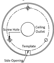
Figure 2-8 Drill Template
