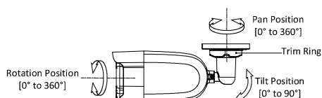
Figure 2-10 3-Axis Adjustment
