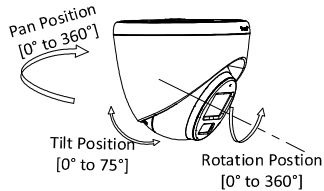
Figure 2-9 3-Axis Adjustment
