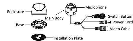
Figure 1-3 Overview of Type III Camera
