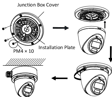
Figure 2-10 Fix the Camera to the Junction Box
