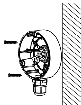
Figure 2-4 Secure the Junction Box on the Wall
