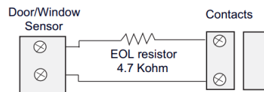
Figure 2: External Contact Wiring
