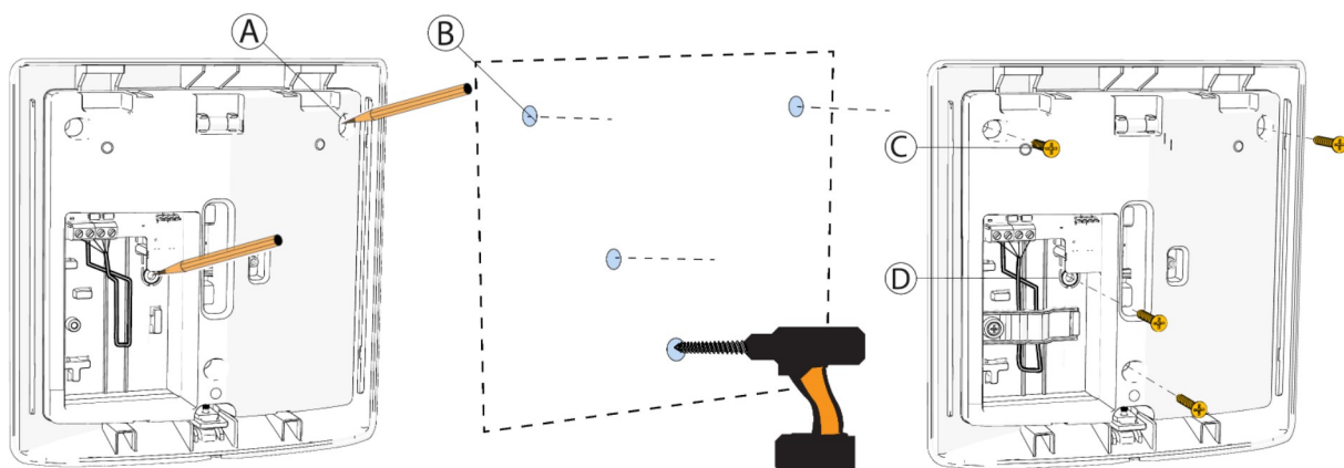
Figure 5: Device screw installation
