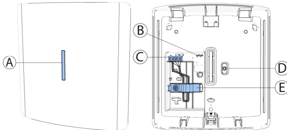
Figure 1: PGPHOST external view
