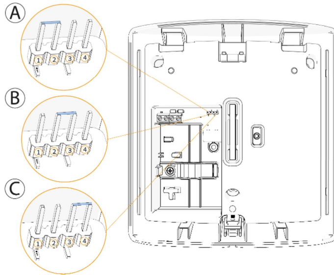
Figure 6: Back and front tamper jumper locations
