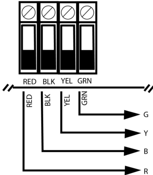
Figure 4: Wiring internal view
