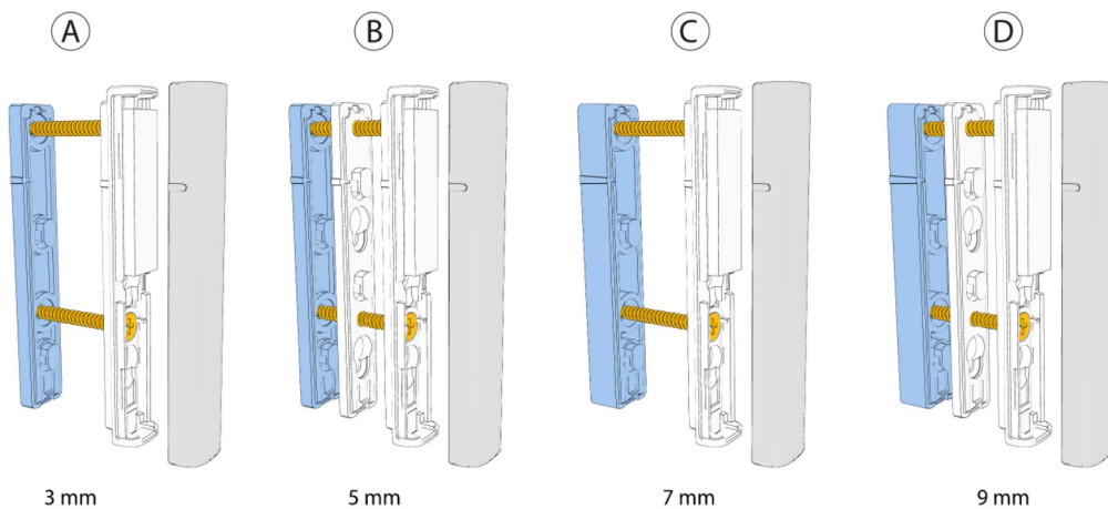
Figure 9: Spacer mounting combinations
