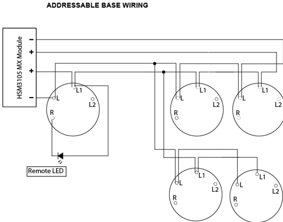
Figure 3: Addressable base wiring diagram
