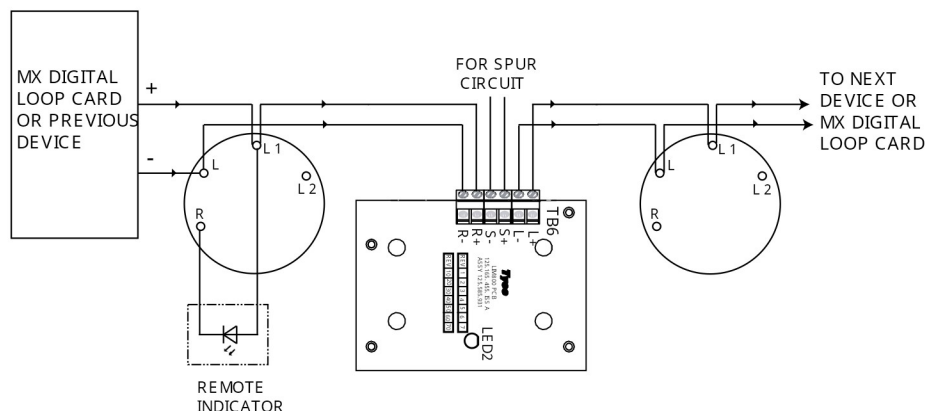
Figure 4: MX920 Wiring
