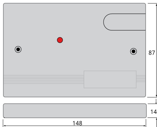
Figure 2: Fascia Plate and Dimensions
