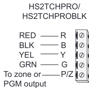
Figure 3 - Wiring
