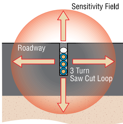
Cutaway of Underground Loop
