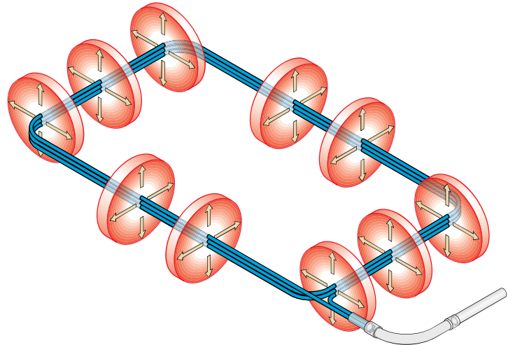
Inductive Field of Sensitivity
