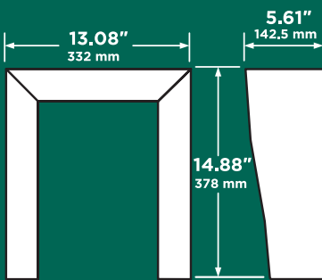
1814-185 Black Hood 1814-180 Stainless Steel Hood
