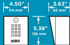
1515 Compact Surface
