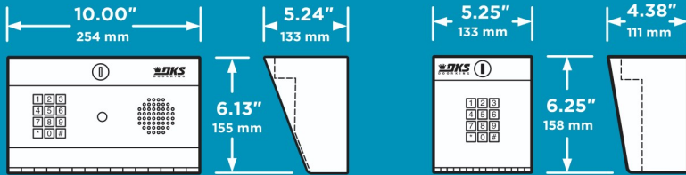
1504 Surface
