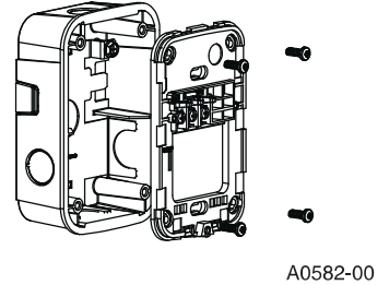
3F. COMPACT WALL MOUNT SURFACE-MOUNT BACK BOX
