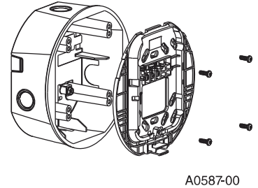
3D. CEILING MOUNT SURFACE-MOUNT BACK BOX
