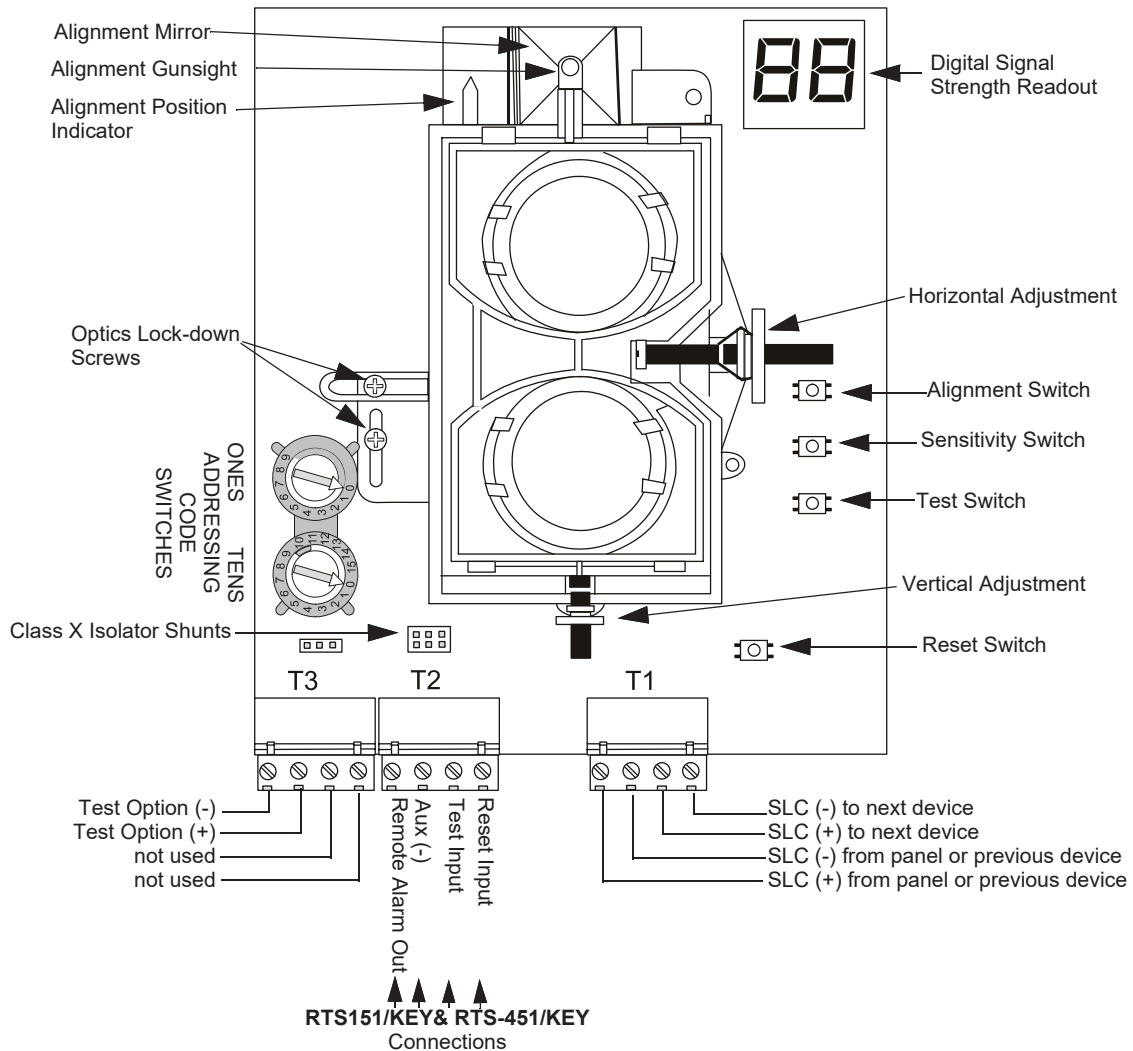
Figure 10.1 SK-BEAM Beam Detector Terminal Block Wiring
