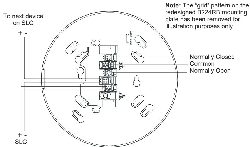
Figure 9.6 Wiring of a B224RB Relay Base Mounting Plate
