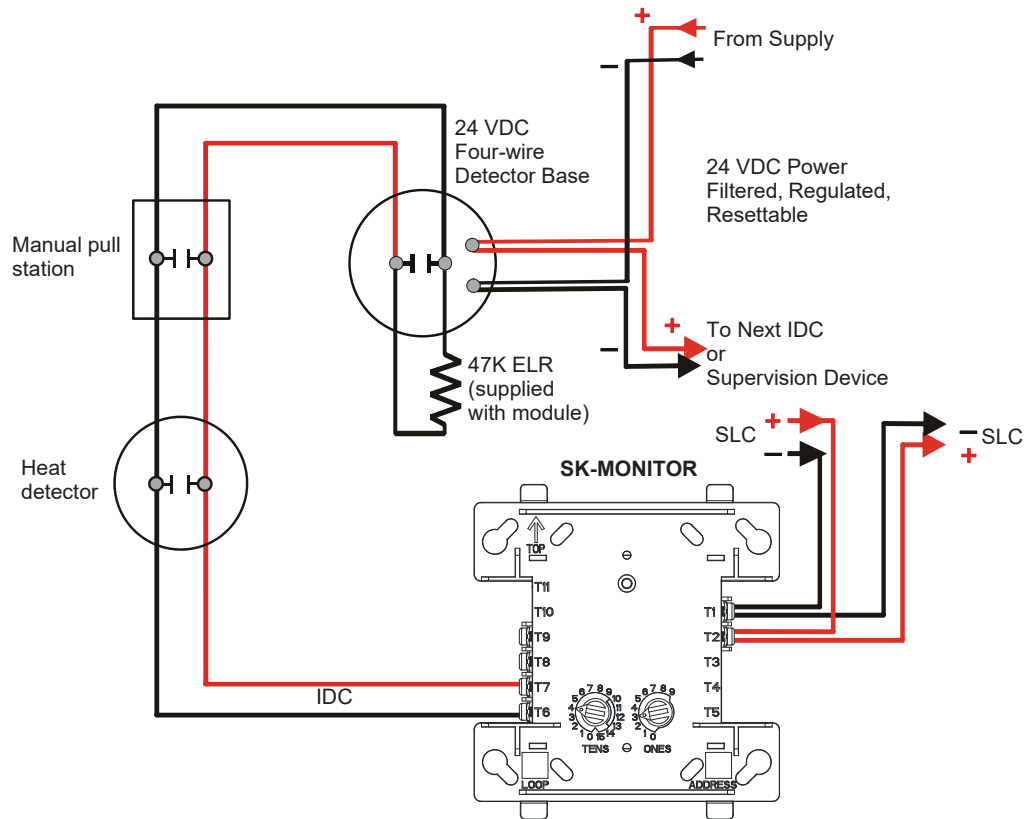
Figure 5.13 Typical Class B IDC Wiring with an SK-MONITOR
