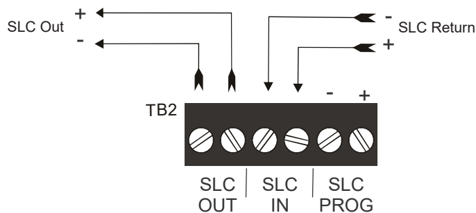
Figure 2.6 Terminal Block
