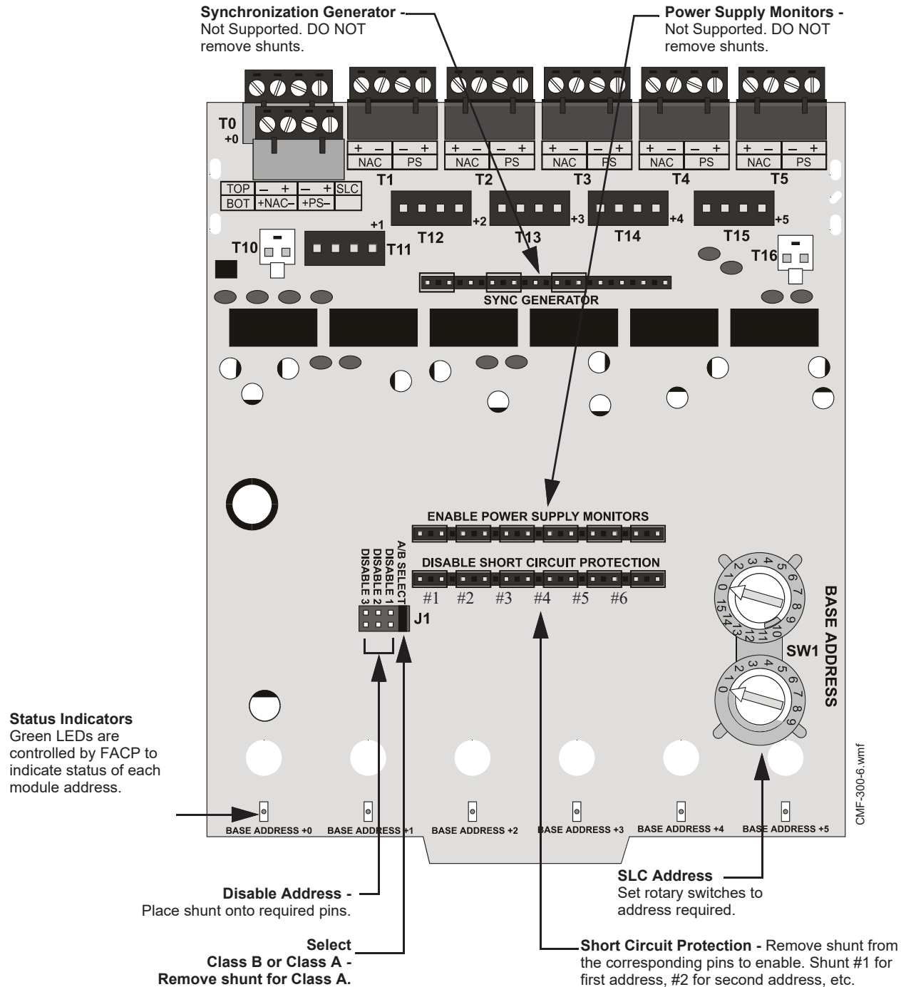
Figure 6.7 SK-CONTROL-6 Control Module Settings
