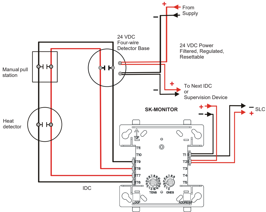
Figure 5.14 Typical Class A IDC Wiring with an SK-MONITOR
