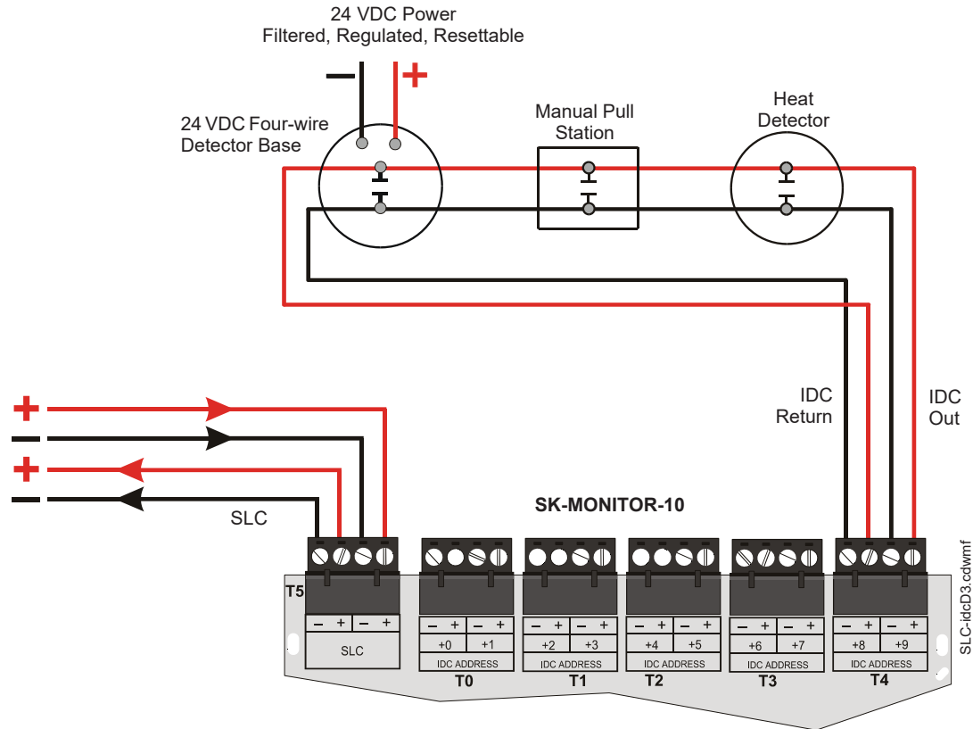
Figure 5.18 Typical Class A IDC Wiring with an SK-MONITOR-10
