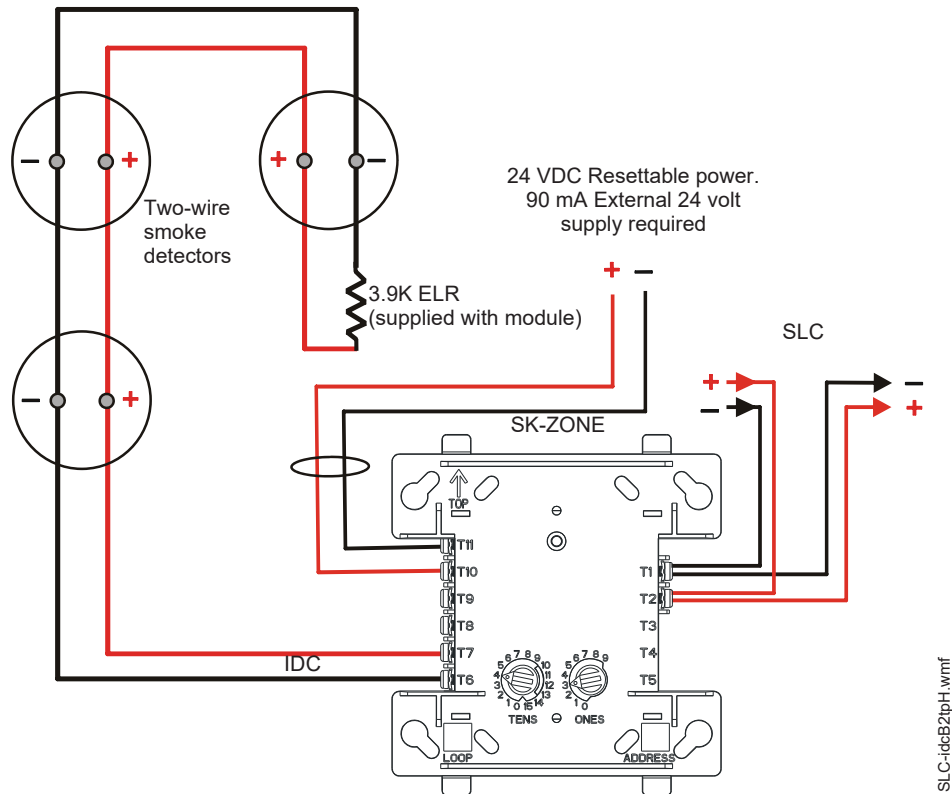
Figure 5.20 Typical Class B IDC Wiring with an SK-ZONE
