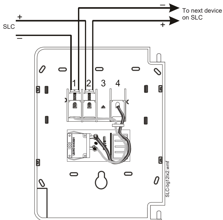
Figure 11.1 Wiring of an SK-PULL-DA Pull Station to an SLC
