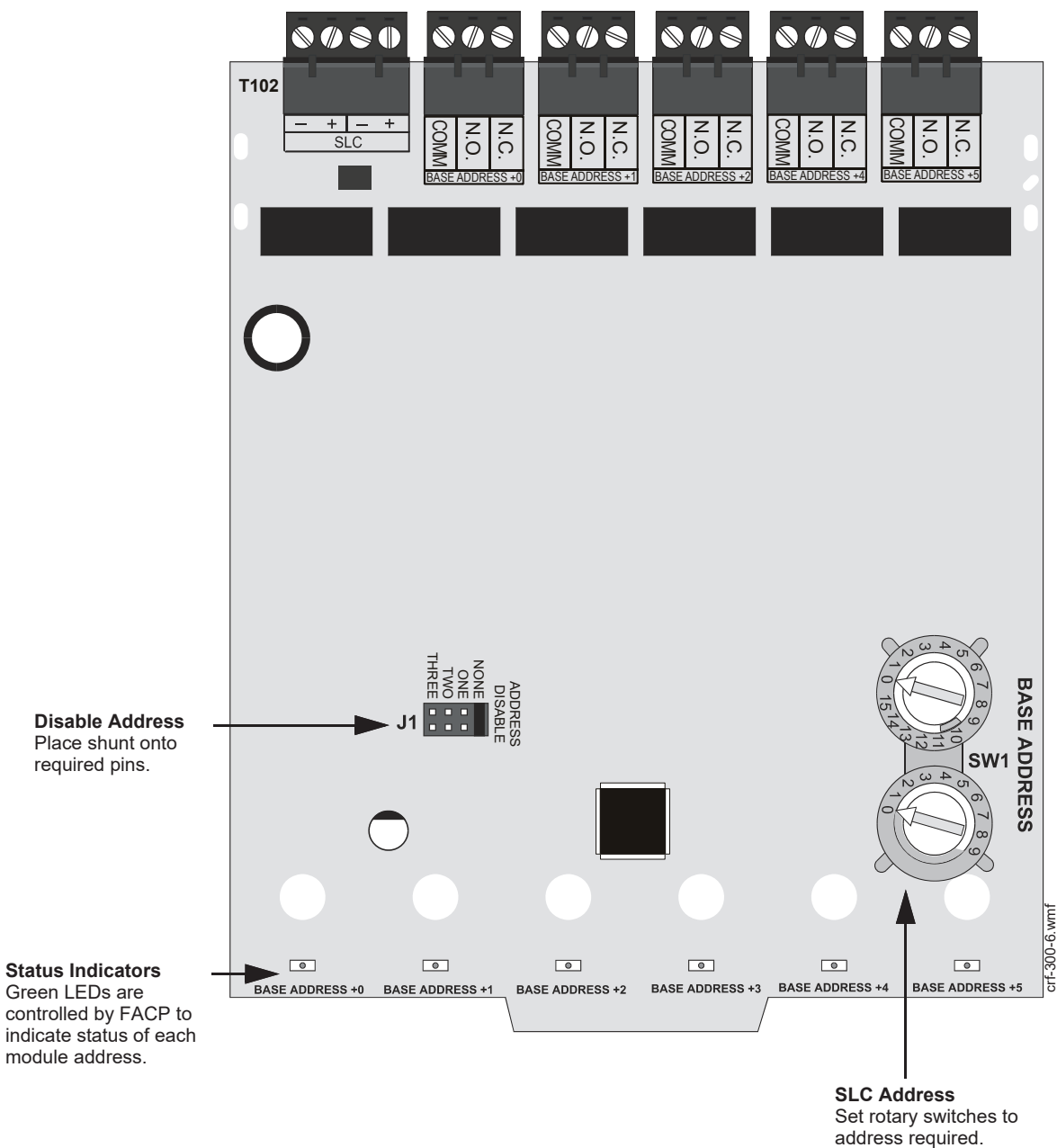
Figure 7.2 SK-RELAY-6 Control Relay Module
