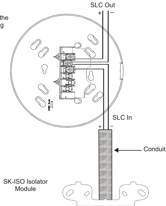
Figure 9.4 Wiring a B224BI Isolator Base Mounting Plate
