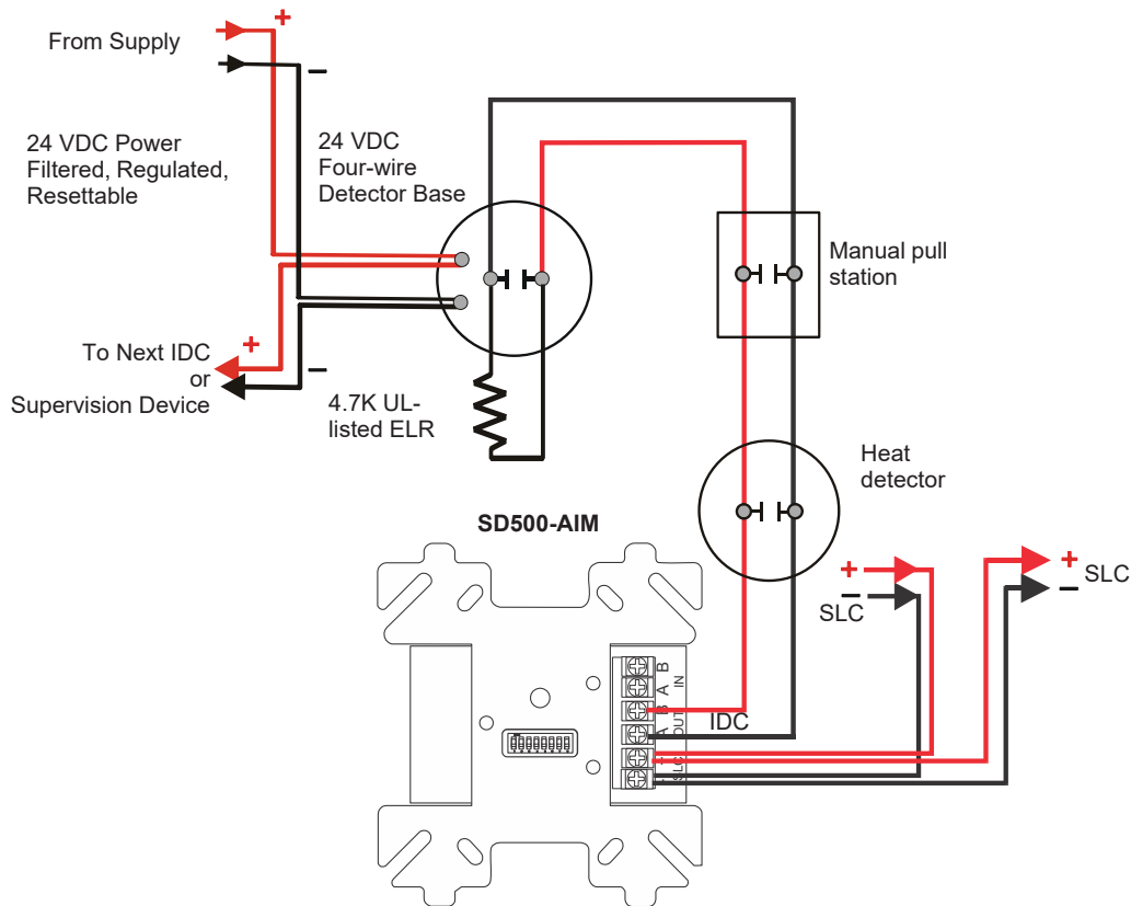
Figure 5.15 Typical Class B IDC Wiring with an SD500-AIM
