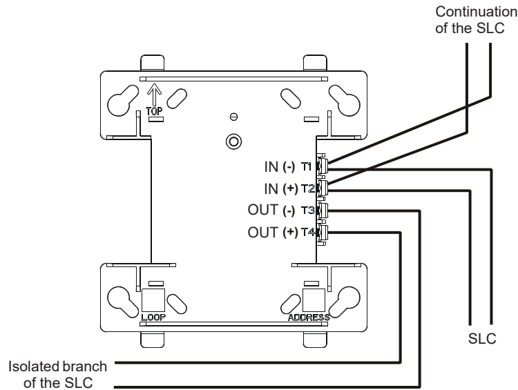
Figure 4.1 Wiring an SK-ISO Module
