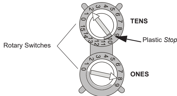
Figure 5.11 Setting an SLC Address on a Multi-Point Module
