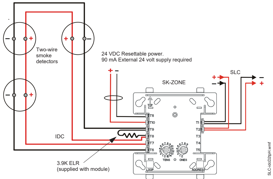
Figure 5.21 Typical Class A IDC Wiring with an SK-ZONE
