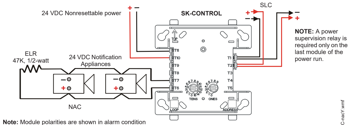
Figure 6.3 NFPA Class B Notification Appliance Circuit with SK-CONTROL
