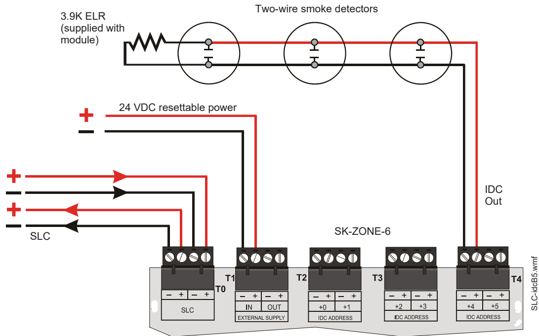
Figure 5.24 Typical Class B IDC Wiring with an SK-ZONE-6
