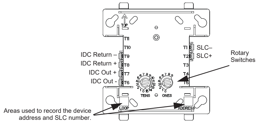
Figure 5.1 SK-MONITOR Monitor Module
