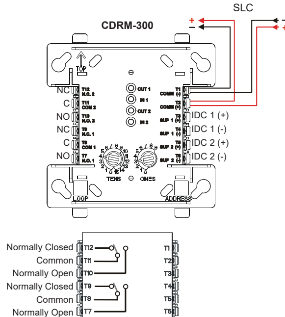
Figure 8.1 SK-RELAYMON-2 Wiring Connections
