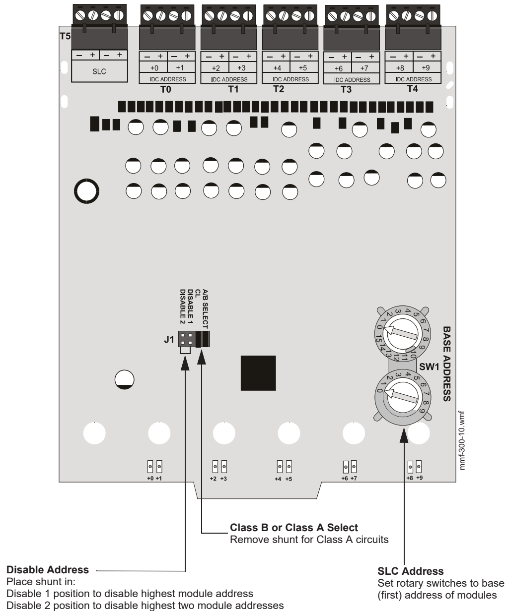
Figure 5.3 SK-MONITOR-10 Monitor Module
