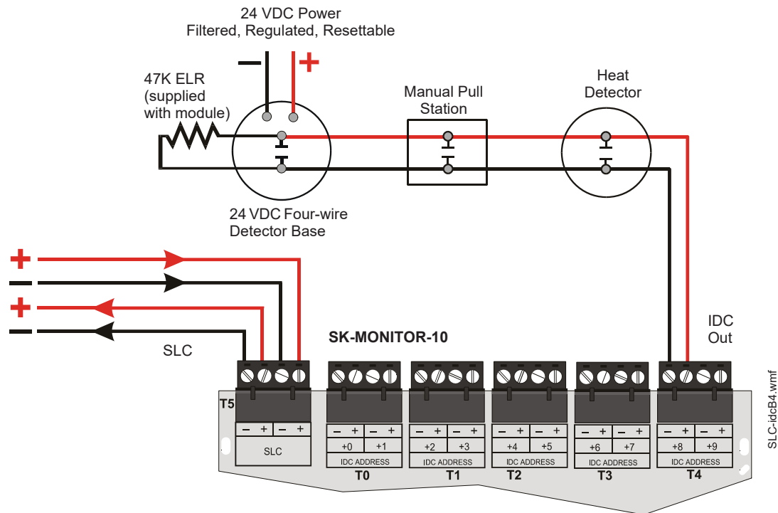
Figure 5.17 Typical Class B IDC Wiring with an SK-MONITOR-10
