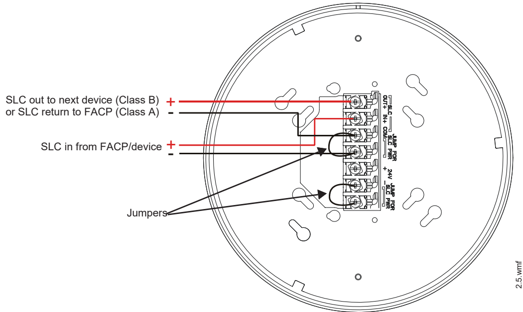
Figure 9.11 WSK-WGI Powered by the SLC
