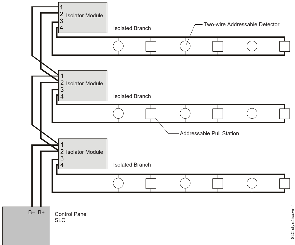
Figure 4.4 NFPA Class B SLC Using SK-ISO and SD500-LIM Isolator Module
