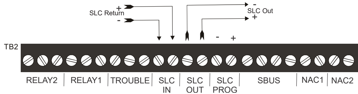
Figure 2.5 6700 Terminal Block
