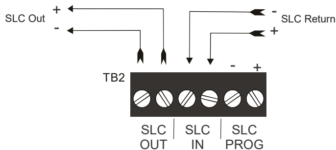
Figure 2.7 Terminal Block
