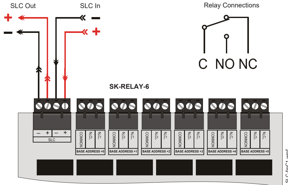
Figure 7.3 SK-RELAY-6 Wiring Connections
