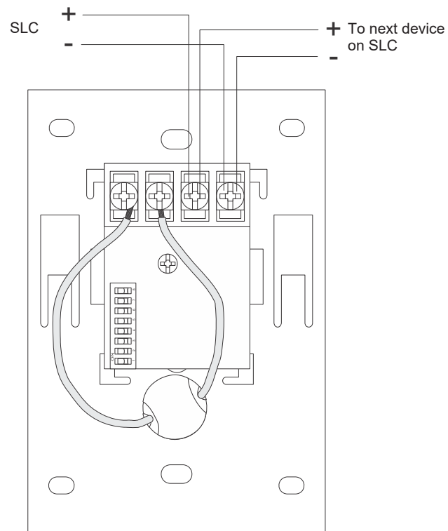
Figure 11.3 Wiring of an SD500-PS/DA Pull Station to an SLC
