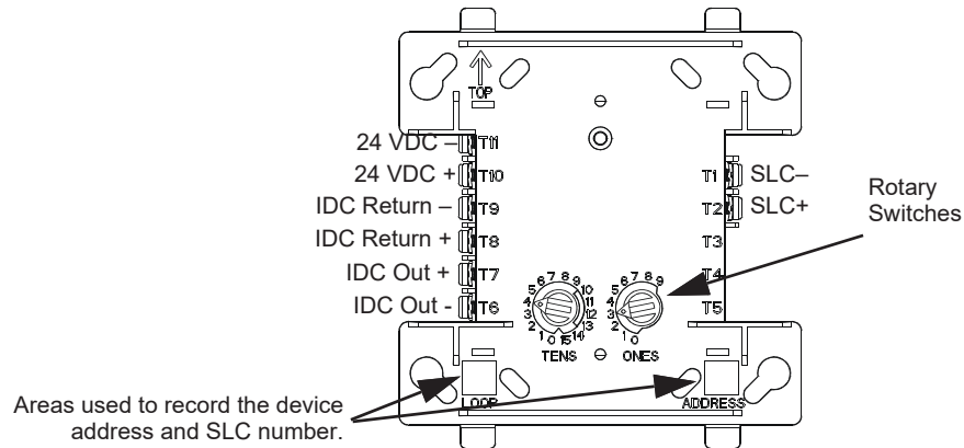
Figure 5.4 SK-ZONE Interface Module
