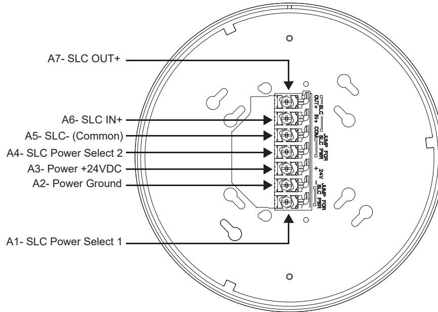
Figure 9.10 WSK-WGI Mounting Plate - Terminal Layout
