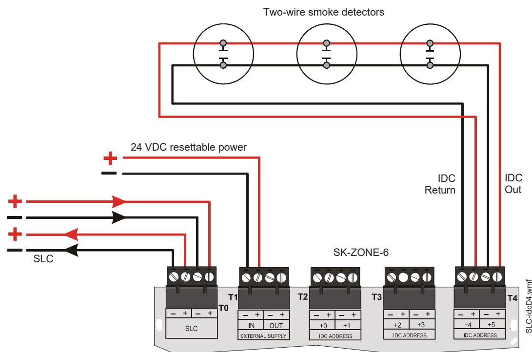
Figure 5.25 Typical Class A IDC Wiring with an SK-ZONE-6
