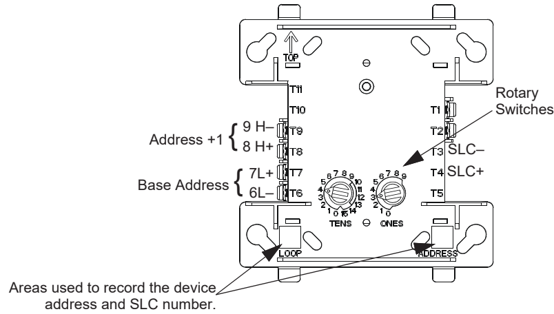
Figure 5.7 SK-MONITOR-2 Dual Monitor Module
