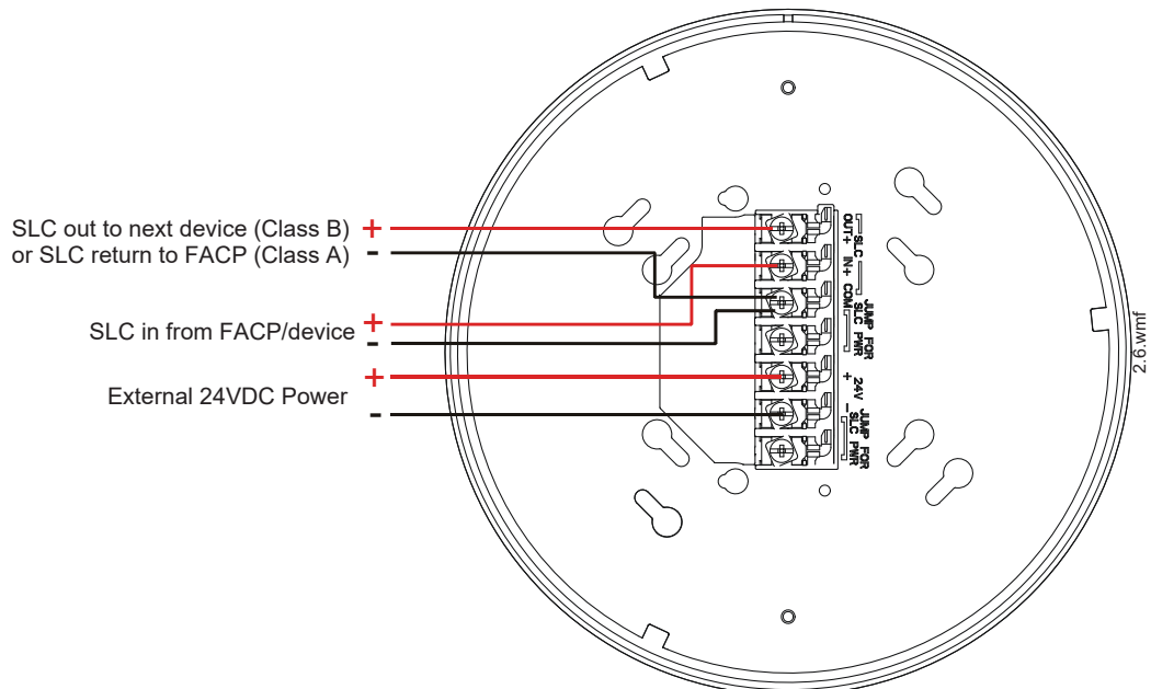
Figure 9.12 WSK-WGI Powered by a Regulated, External Source
