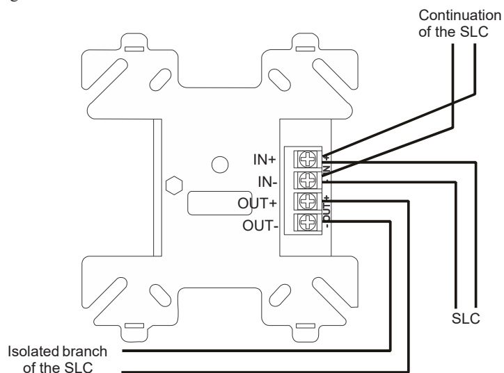
Figure 4.3 Wiring an SD500-LIM
