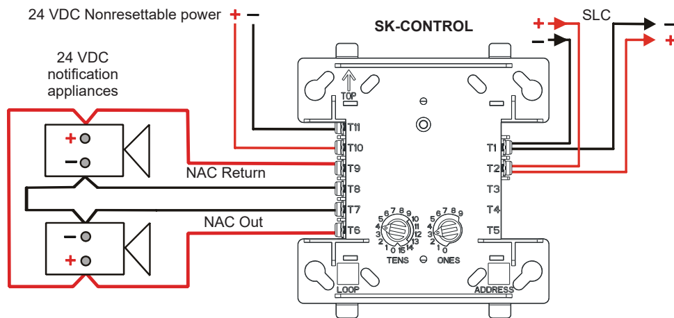
Figure 6.5 NFPA Class A Notification Appliance Circuit with SK-CONTROL
