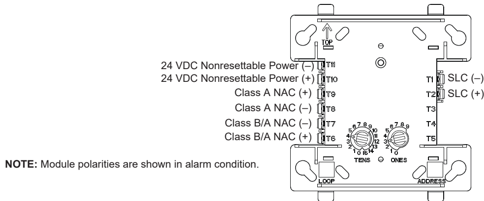
Figure 6.1 SK-CONTROL Wiring Connections
