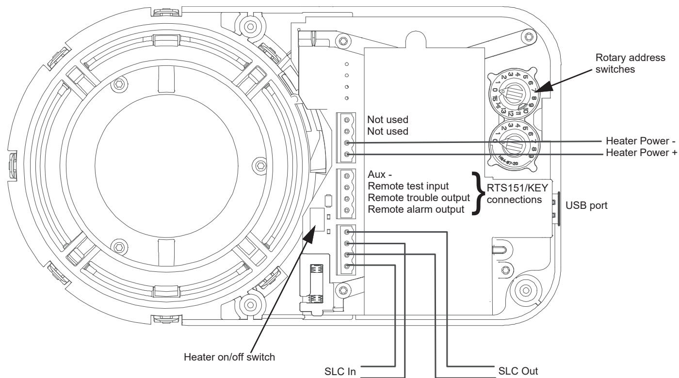
Figure 10.2 OSI-RI-SK Beam Detector Terminal Block Wiring
