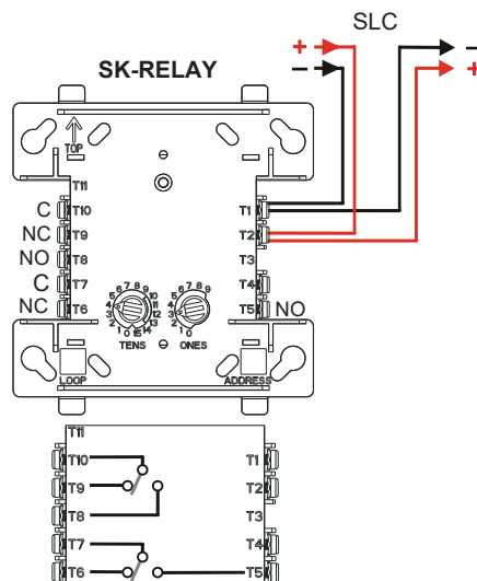
Figure 7.1 SK-RELAY Wiring Connections
