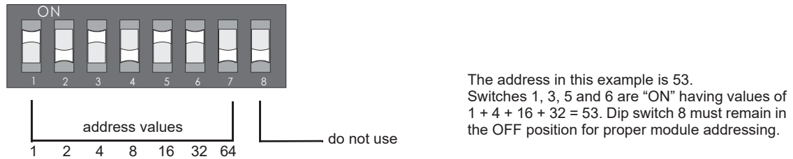
Figure 5.12 Setting an SLC Address on an SD Module
