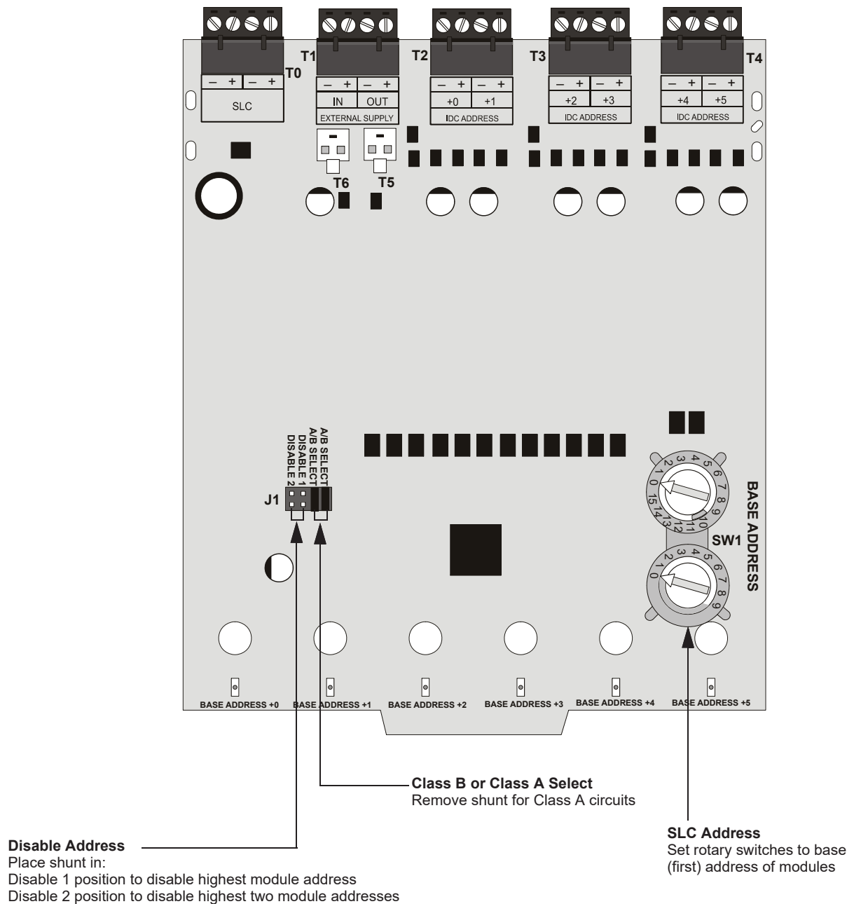
Figure 5.6 SK-ZONE-6 Interface Module
