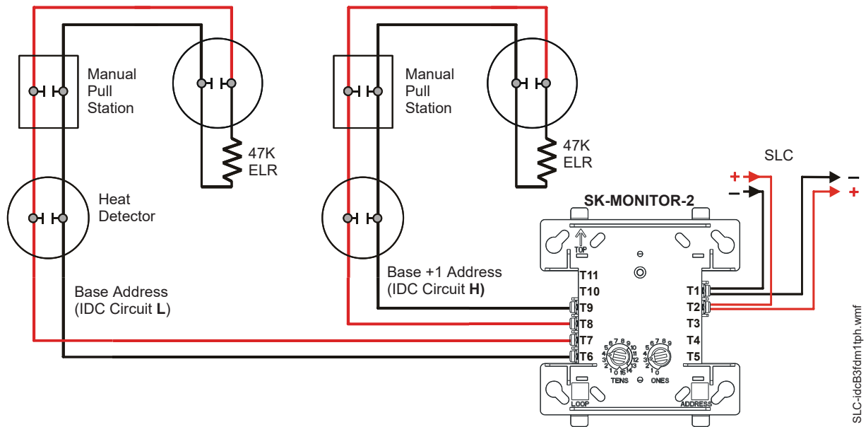
Figure 5.19 Typical Class B IDC Wiring with an SK-MONITOR-2
