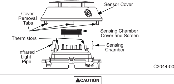
FIGURE 4. CLEANING THE PTIR DETECTOR
