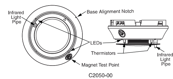
FIGURE 4. CLEANING THE PTIR DETECTOR
