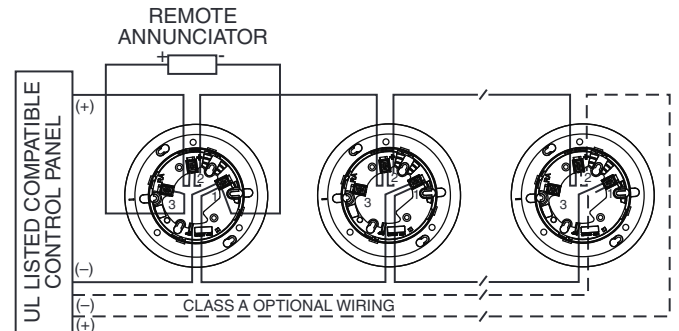
FIGURE 1. WIRING DIAGRAM
