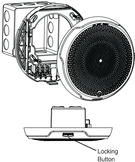
FIGURE 5. CEILING SPEAKER
