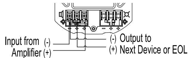
FIGURE 1. WIRING DIAGRAM AND WIRING TERMINALS
