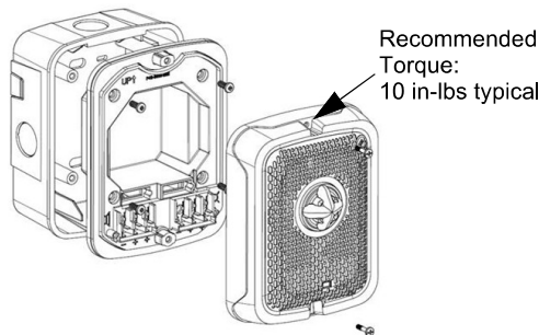
Figure 7 Surface Mounting a Wall Device (SBBSPL/SBBSPWL)
