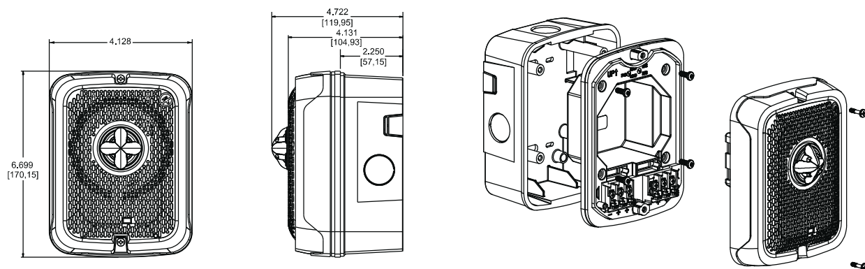
Outdoor Wall Speaker Strobes with Surface Mount Back Box (SBBSPRL/SBBSPWL)
