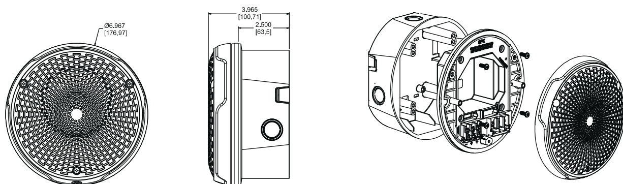
Outdoor Ceiling Speaker with Surface Mount Back Box (SBBCLRL/SBBCWL)
