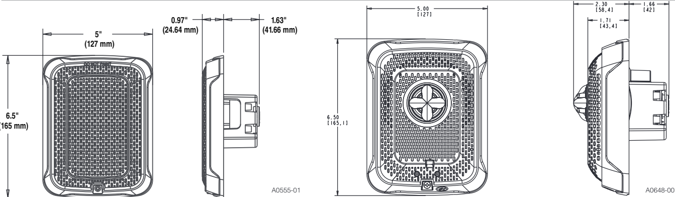
Wall-Mount Speaker
