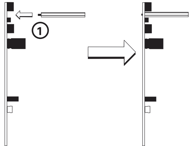
FIGURE 6A: INSTALLATION OF ISO-6 MODULE IN A REAR CHASSIS POSITION, METHOD TWO
