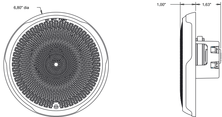
Ceiling Speaker
