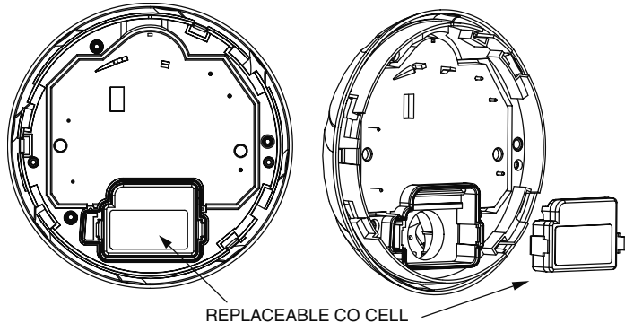
FIGURE 1: CO SENSOR REPLACEMENT
