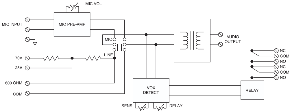
VAR1 Block Diagram
