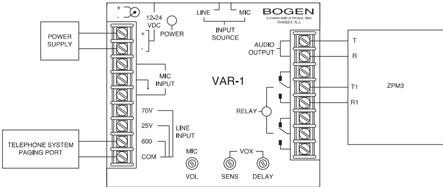
VAR1 Block Diagram
