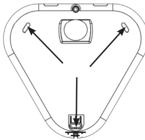
Mounting Holes
