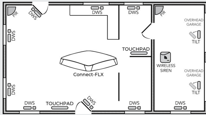
Typical Burglary Protection Installation
