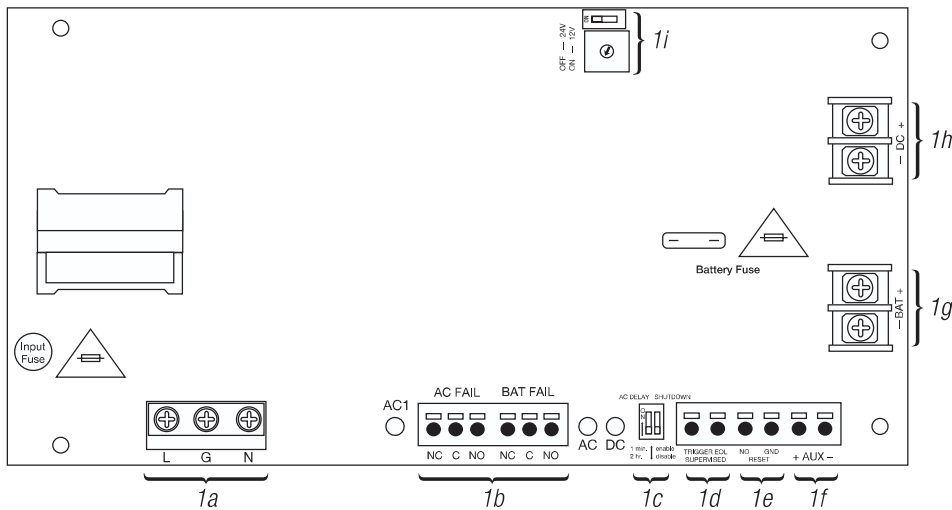
Fig. 1 - eFlowNB Configuration
