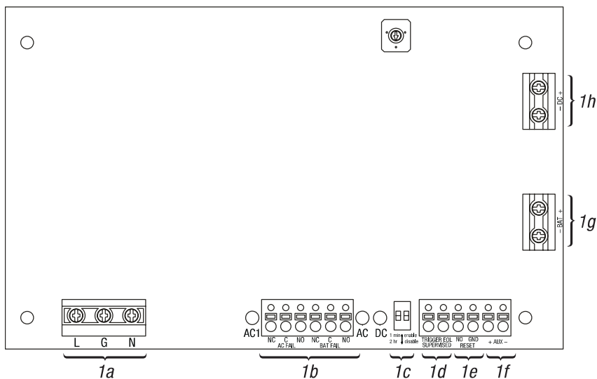
Fig. 1 - eFlow102N Board Configuration
