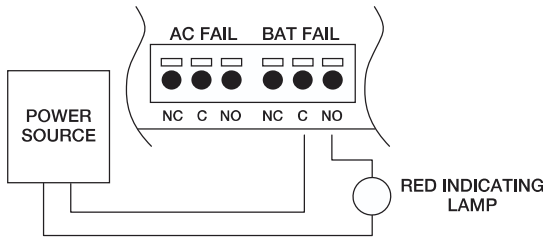
Fig. 2 - Battery Trouble Indication For Canadian use, a red indicating lamp must be visible from the exterior of this enclosure. Wire one leg of a UL Listed, power-limited power source to the indicating lamp. Wire the second leg of the power source to the indicating lamp in series with the battery fail relay contact terminals marked [BAT FAIL - C, NO] (Fig. 2, pg. 6).
