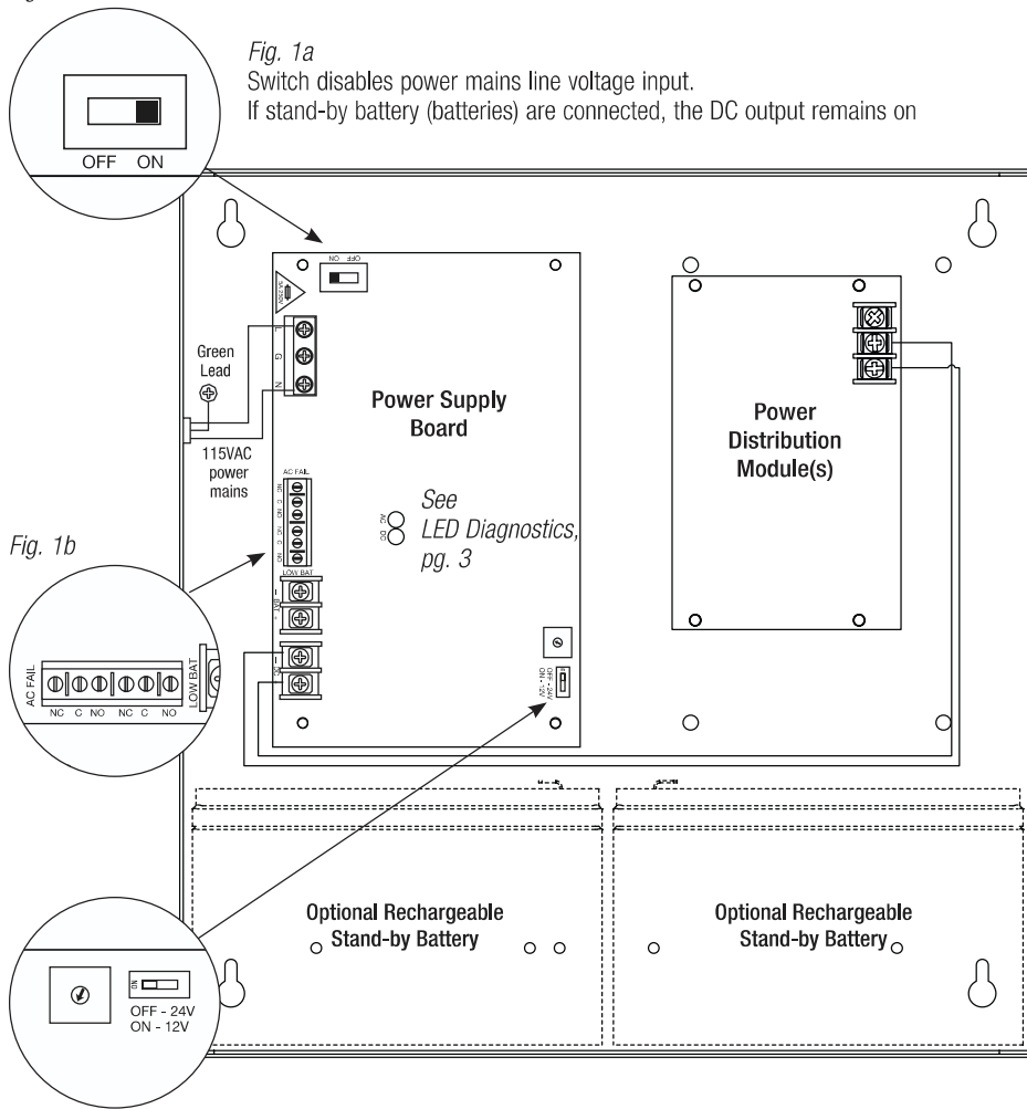
Fig. 1c SW1 12VDC - ON 24VDC - OFF
